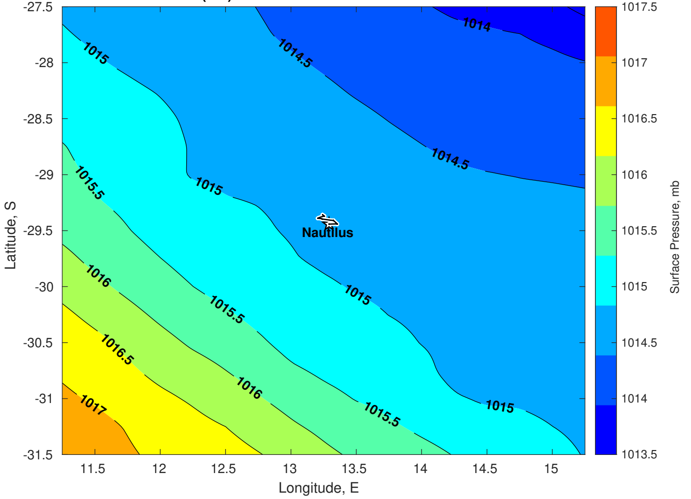
Surface Pressure (mb) for Nautilus at 23-Feb-2025 00:00:00
