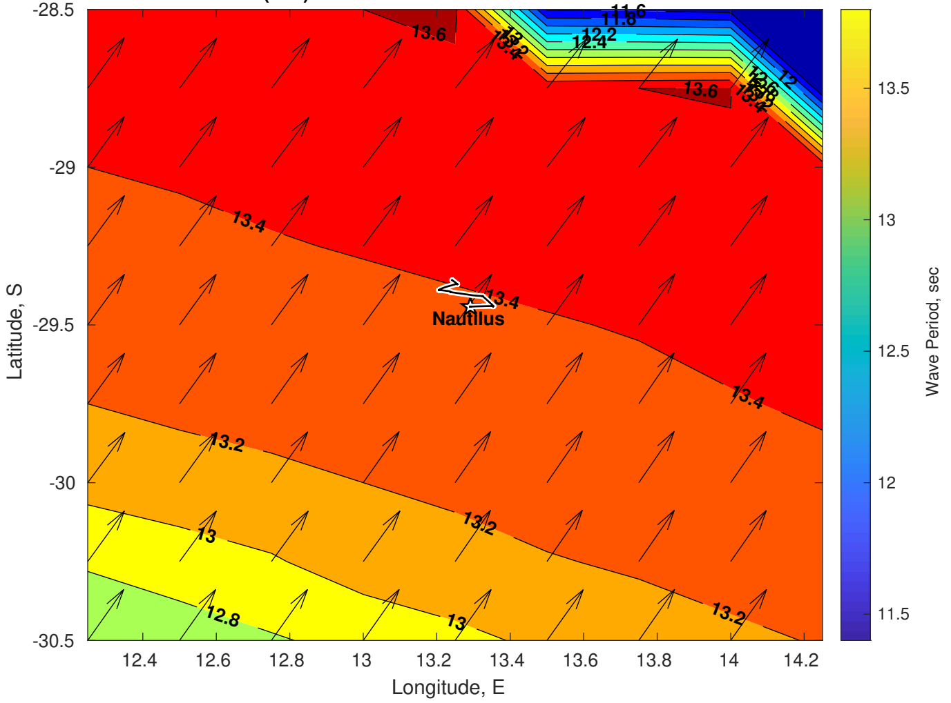
Wave Period (sec) for Nautilus at 23-Feb-2025 09:00:00
