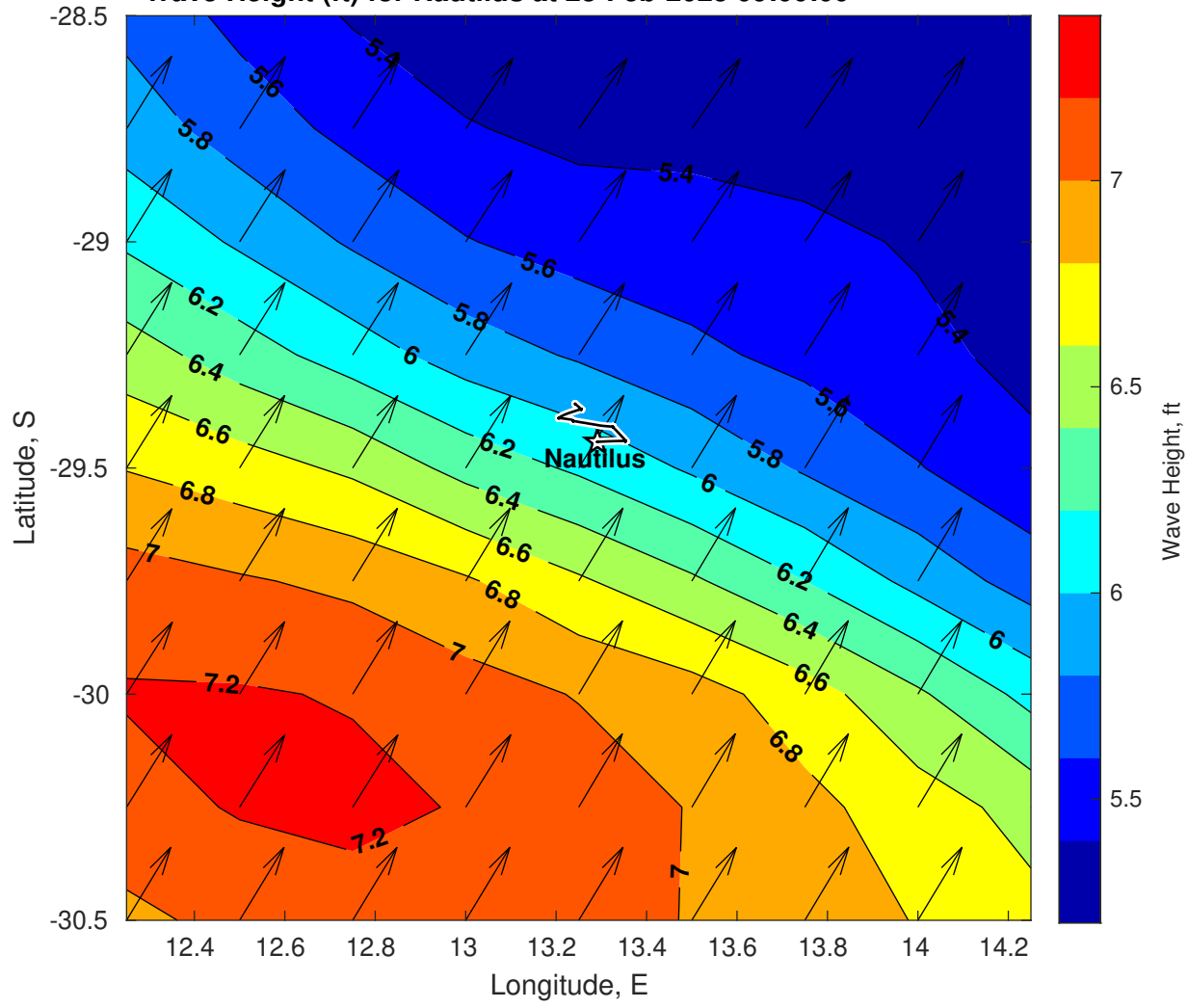
Wave Height (ft) for Nautilus at 23-Feb-2025 09:00:00
