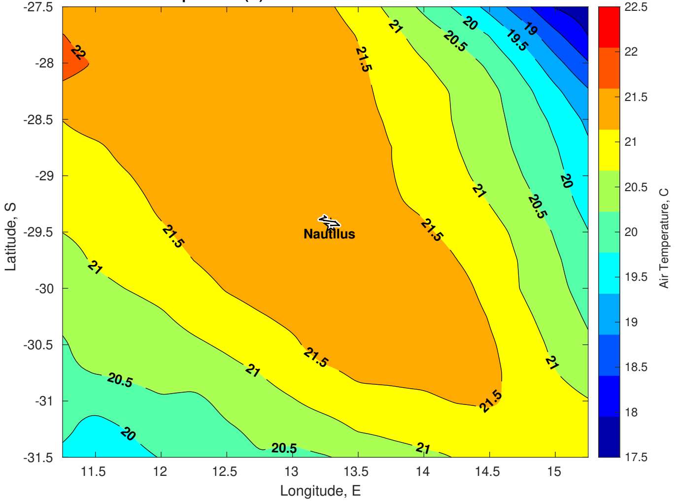
Air Temperature (C) for Nautilus at 23-Feb-2025
