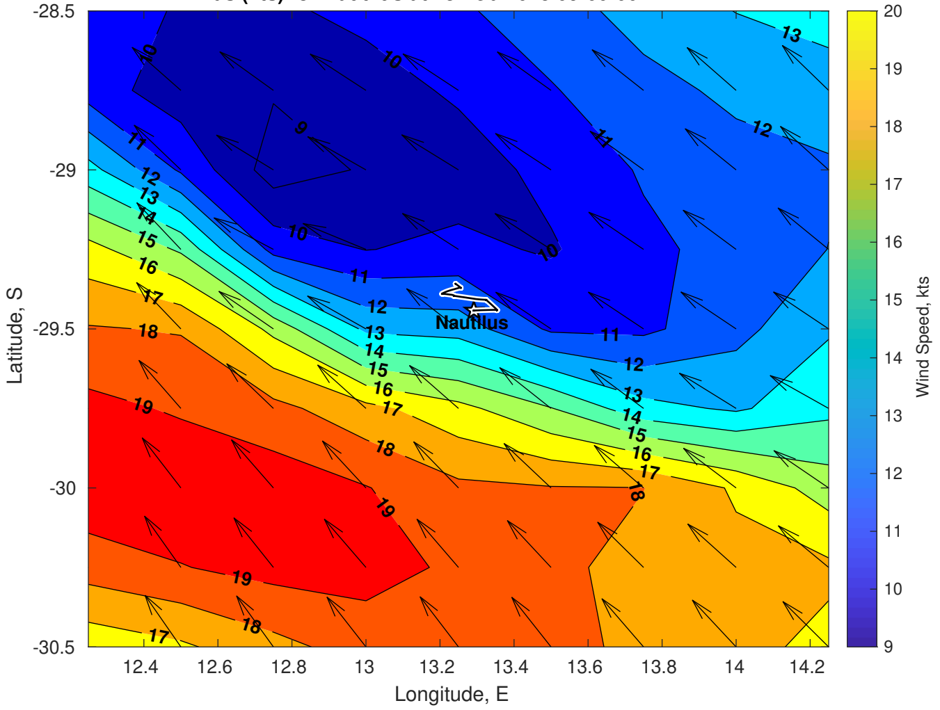
Winds (kts) for Nautilus at 23-Feb-2025 09:00:00
