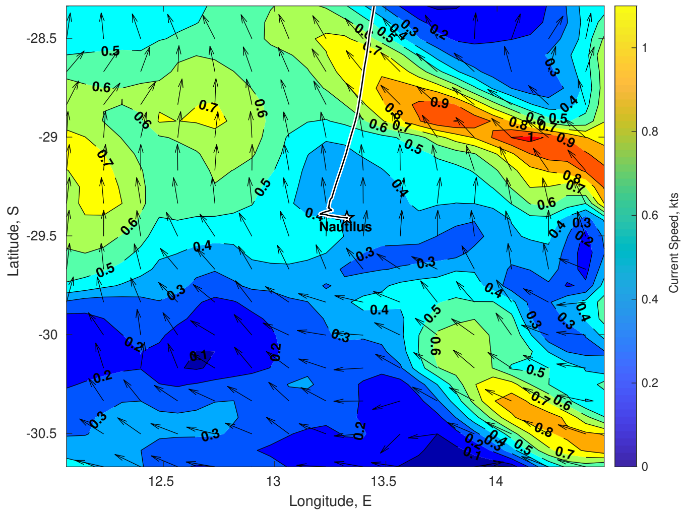
Surface Currents for Nautilus at 22-Feb-2025 00:00:00
