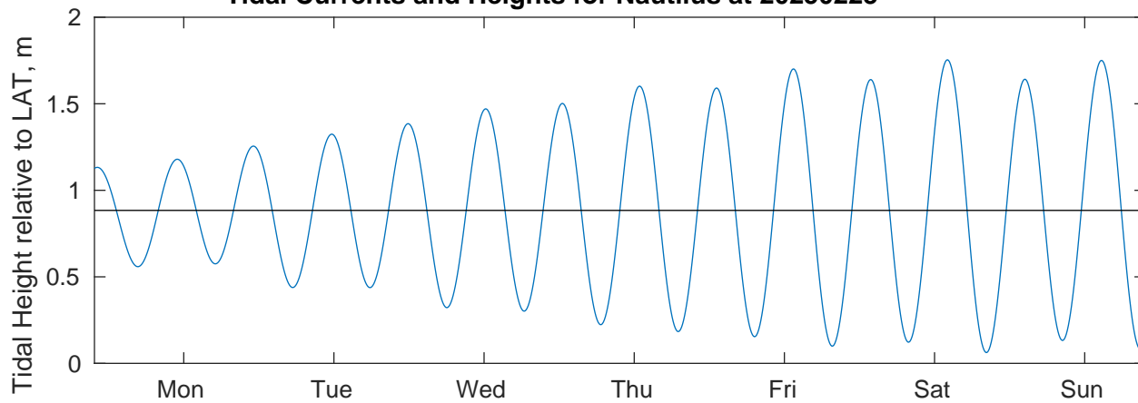
Tidal Currents and Heights for Nautilus at 20250223
