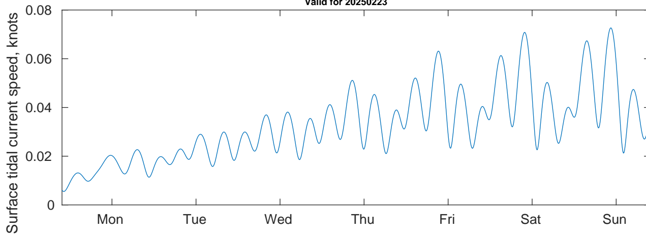
Tidal Currents and Heights for Nautilus at 20250223
