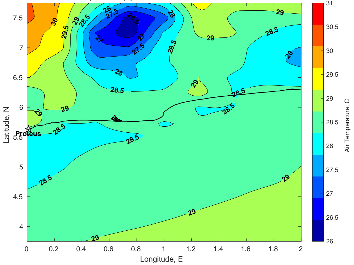
Air Temperature (C) for Proteus at 23-Feb-2025
