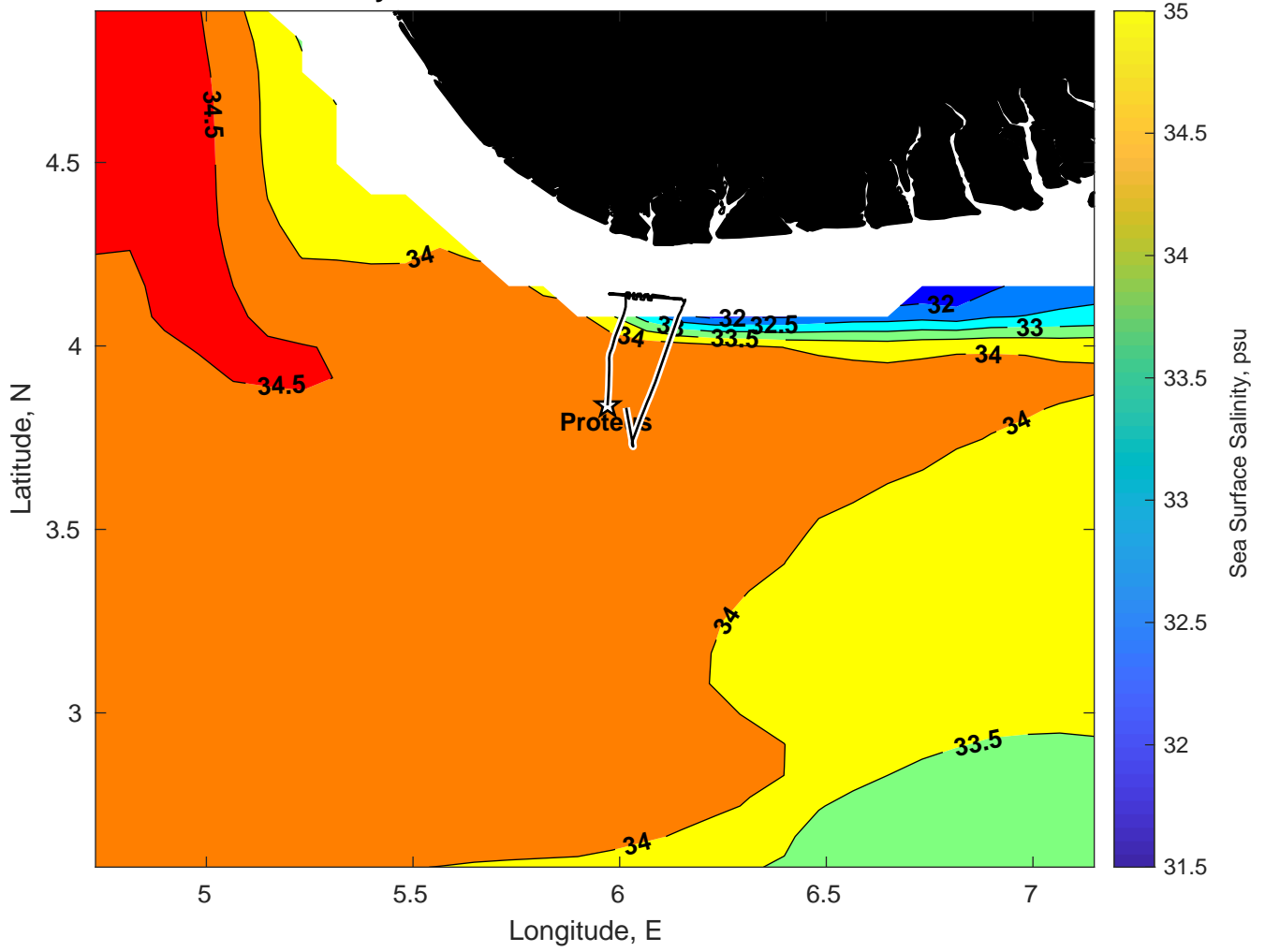
Surface Salinity for Proteus at 22-Feb-2025 00:00:00
