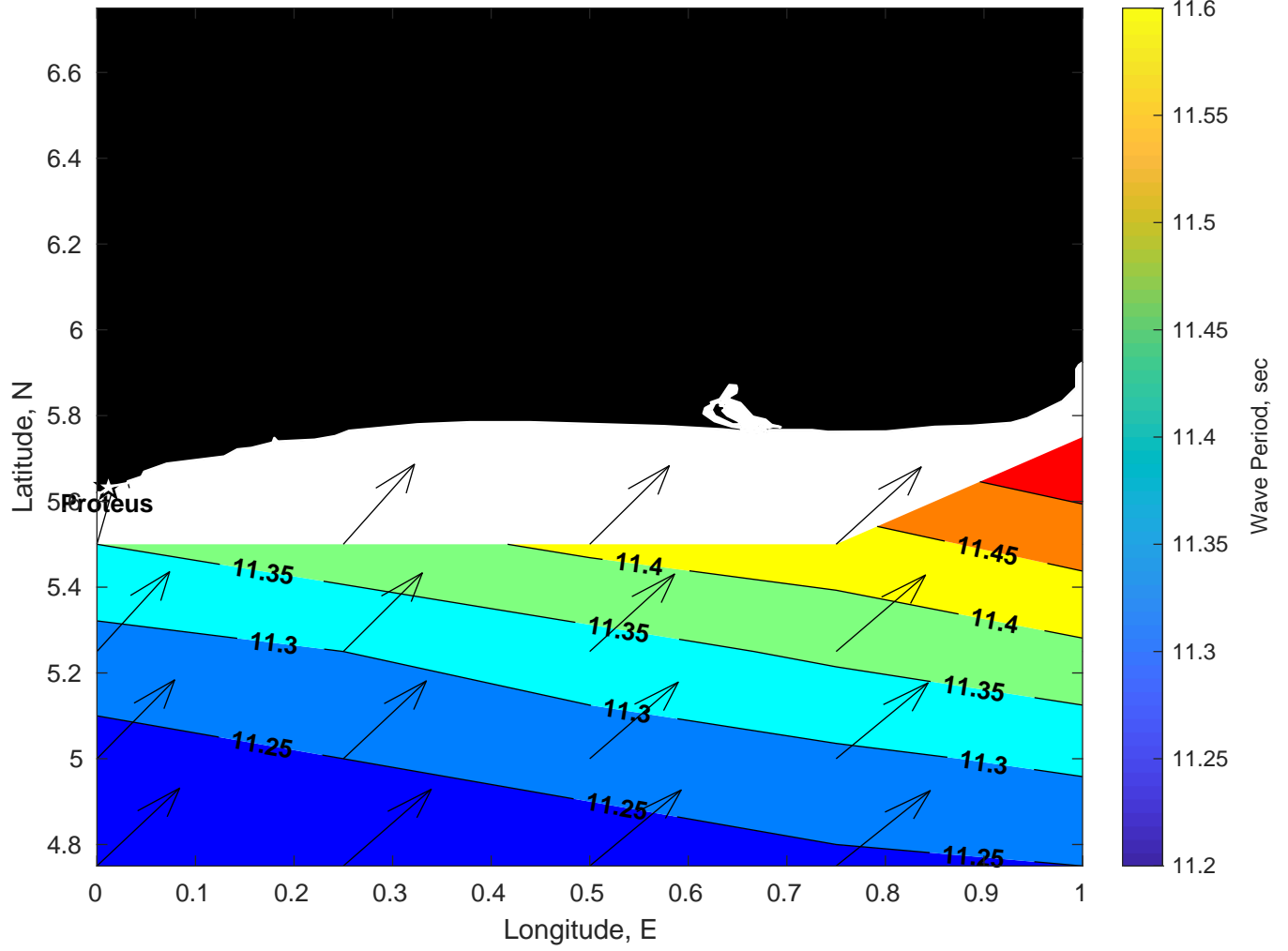
Wave Period (sec) for Proteus at 23-Feb-2025 09:00:00
