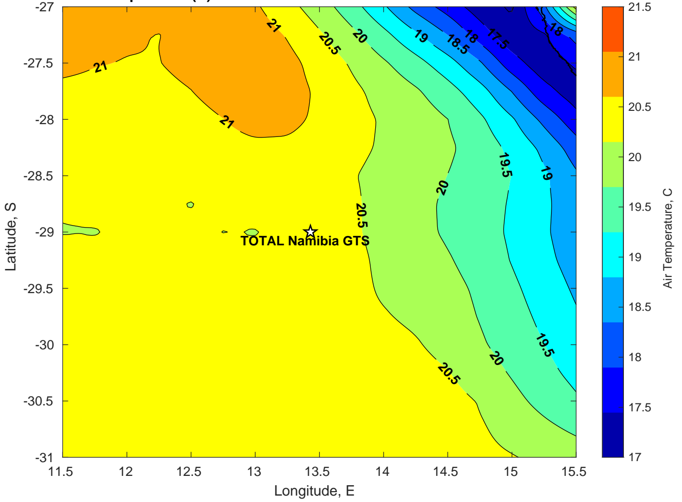
Air Temperature (C) for TOTAL Namibia GTS at 23-Feb-2025
