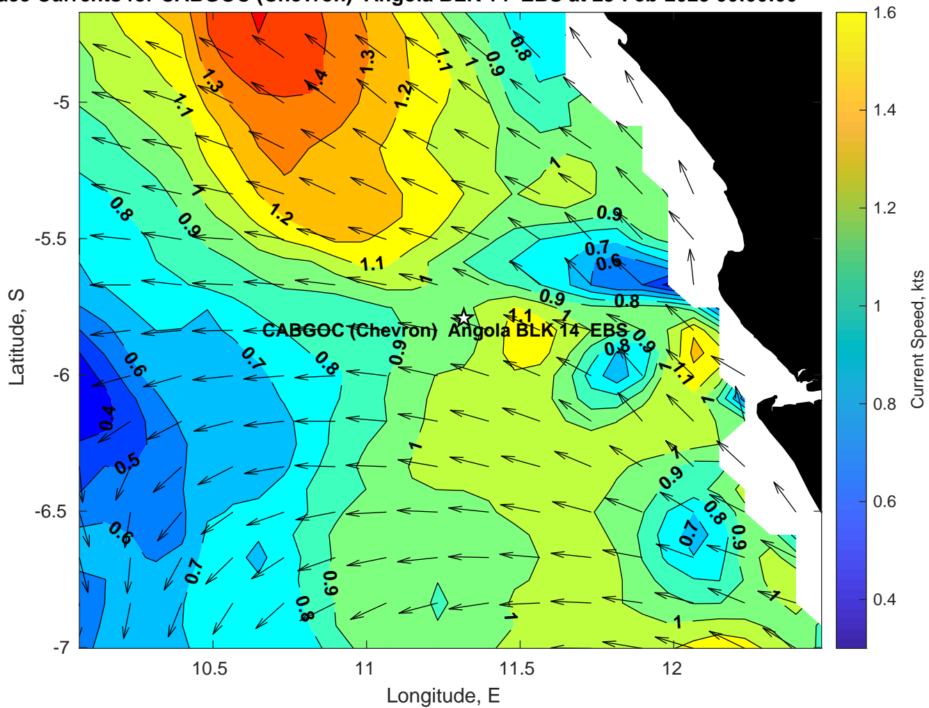
Surface Currents for CABGOC (Chevron) Angola BLK 14 EBS at 23-Feb-2025 00:00:00
