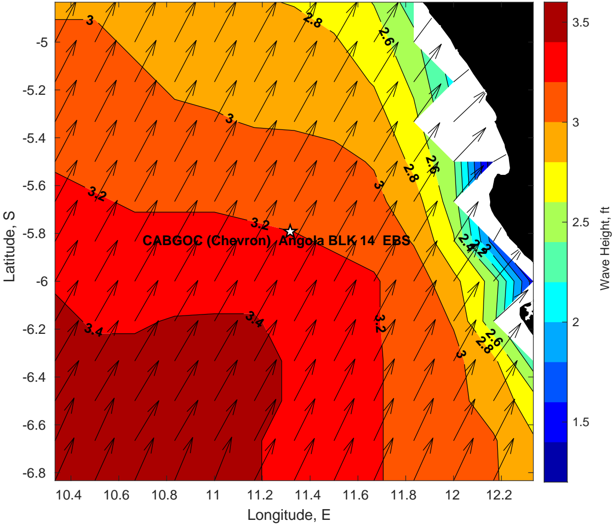
Wave Height (ft) for CABGOC (Chevron) Angola BLK 14 EBS at 24-Feb-2025 09:00:00
