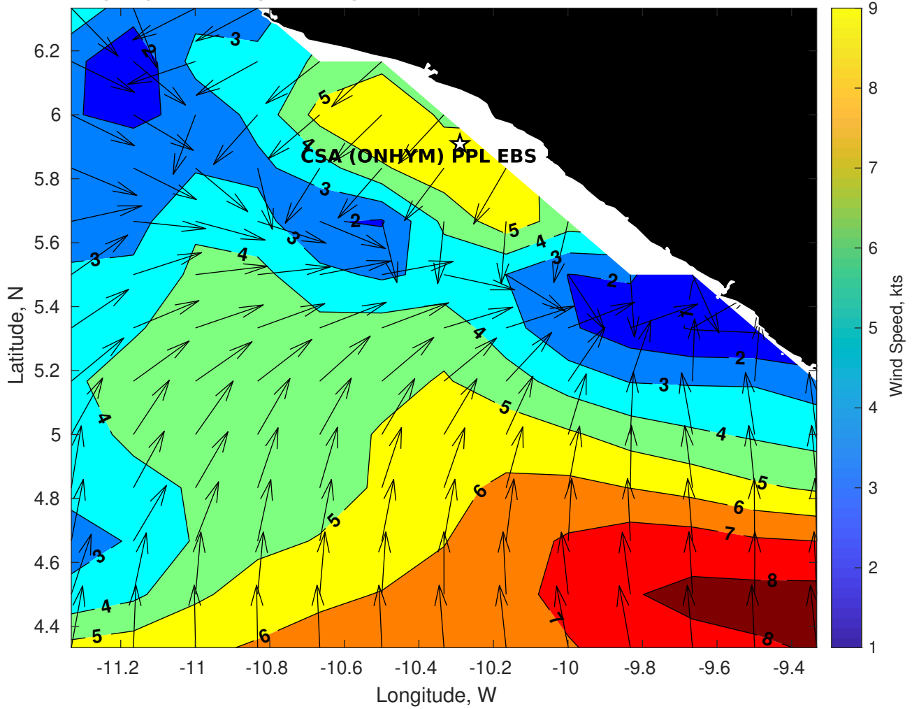
Winds (kts) for CSA (ONHYM) PPL EBS - Liberia at 24-Feb-2025 09:00:00
