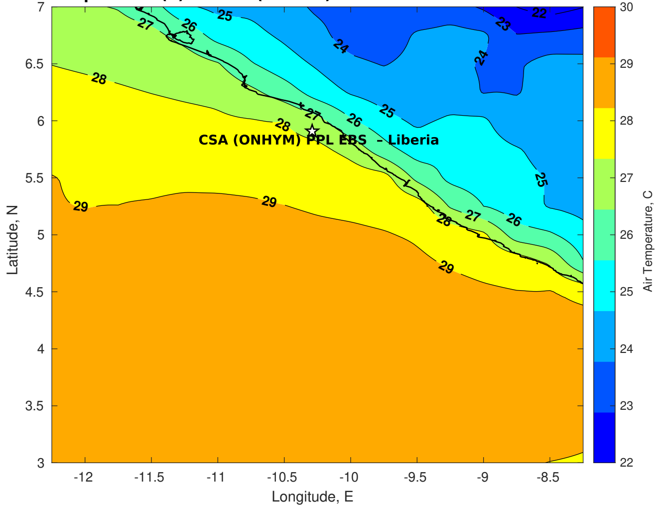
Air Temperature (C) for CSA (ONHYM) PPL EBS - Liberia at 24-Feb-2025
