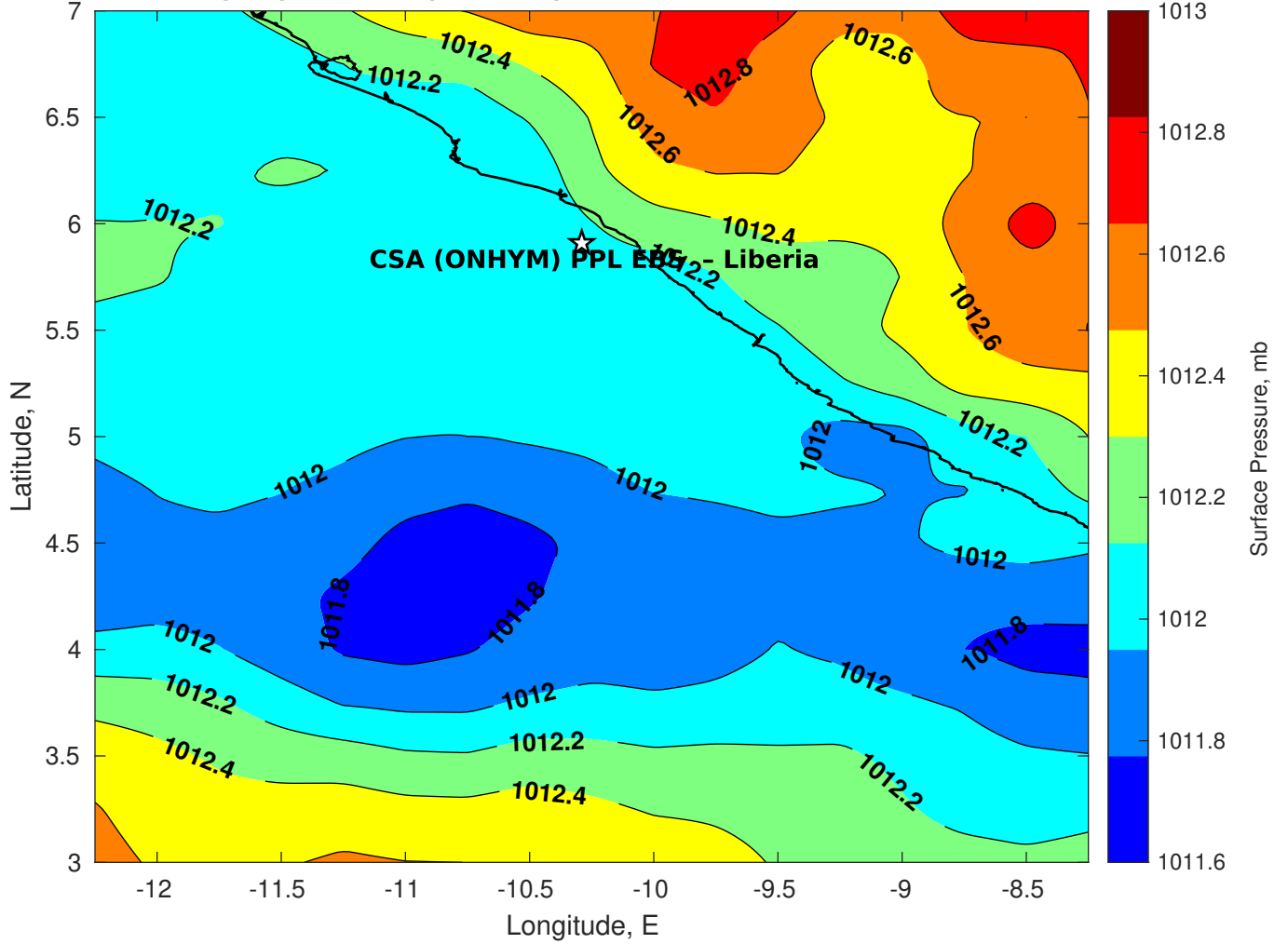
Surface Pressure (mb) for CSA (ONHYM) PPL EBS - Liberia at 26-Feb-2025 00:00:00
