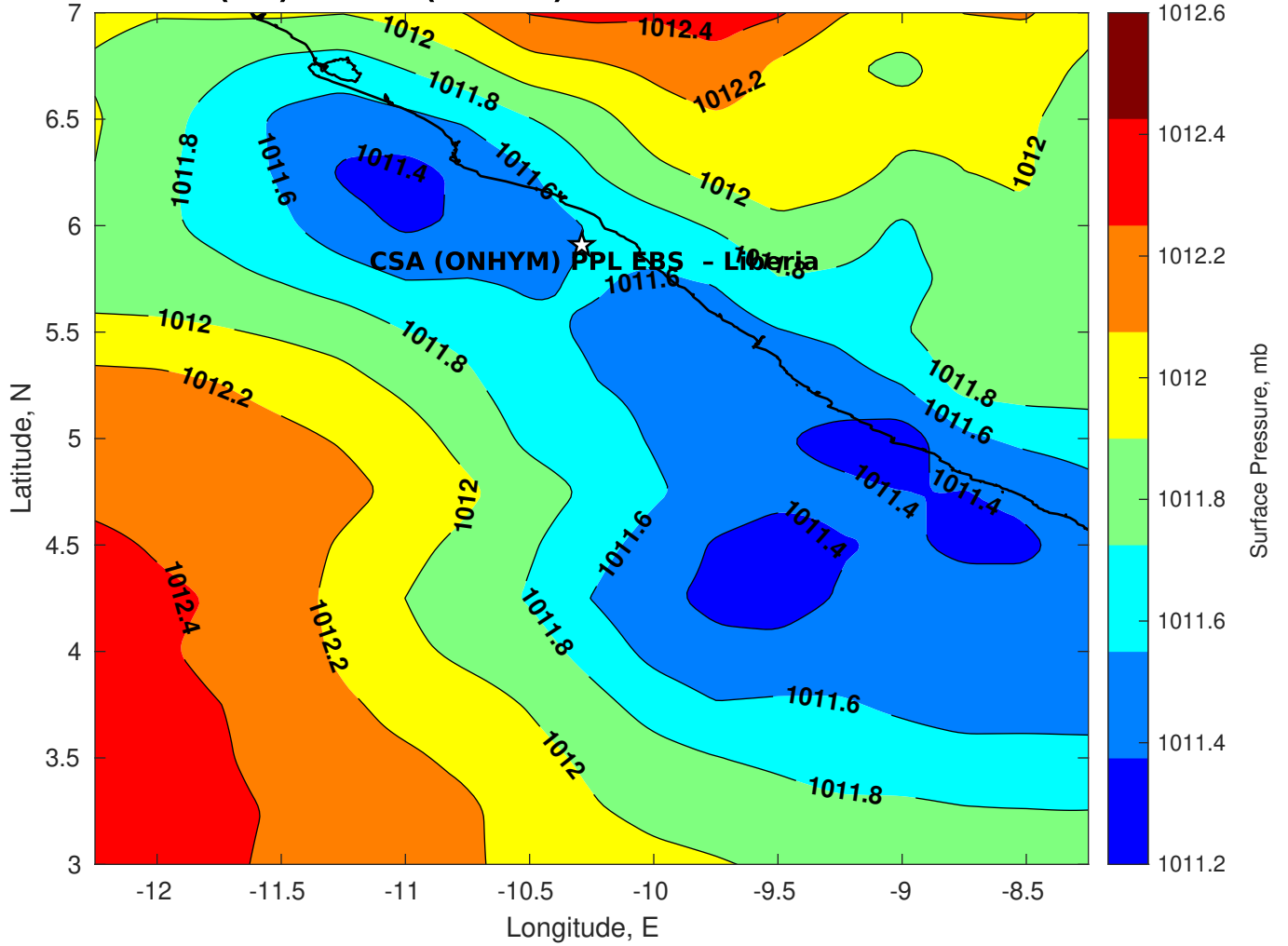
Surface Pressure (mb) for CSA (ONHYM) PPL EBS - Liberia at 25-Feb-2025 00:00:00
