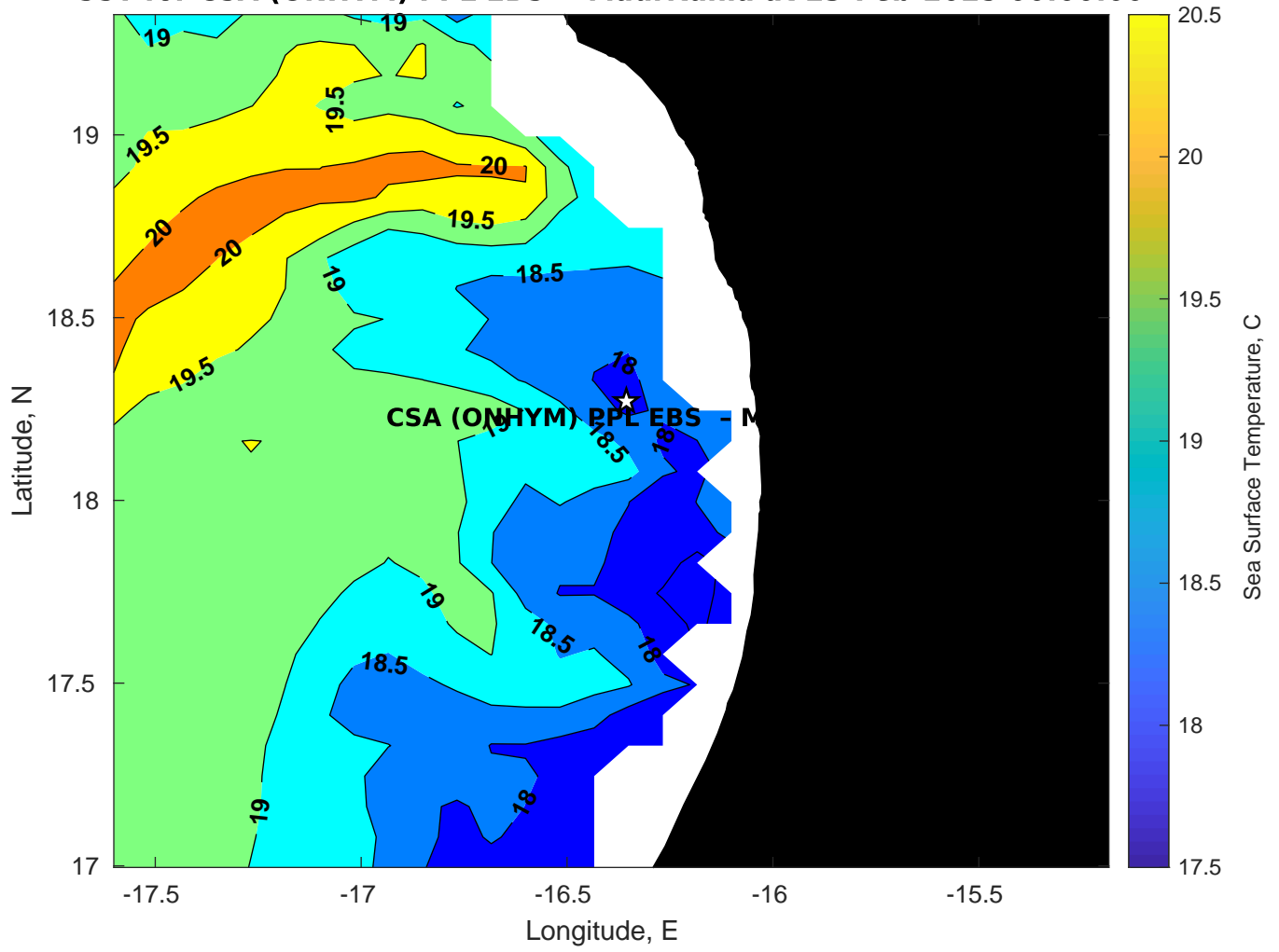
SST for CSA (ONHYM) PPL EBS - Mauritania at 23-Feb-2025 00:00:00
