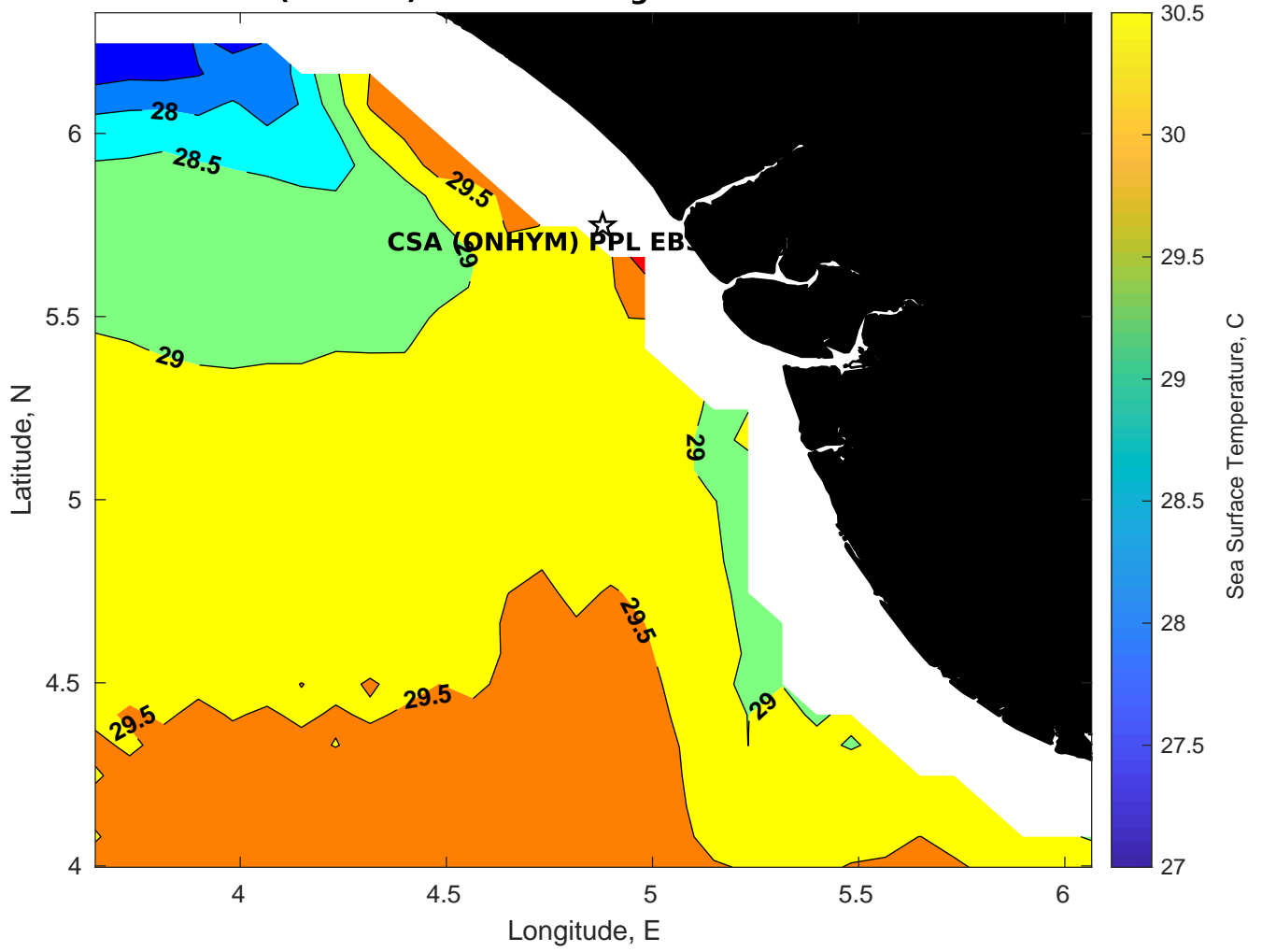
SST for CSA (ONHYM) PPL EBS - Nigeria at 23-Feb-2025 00:00:00
