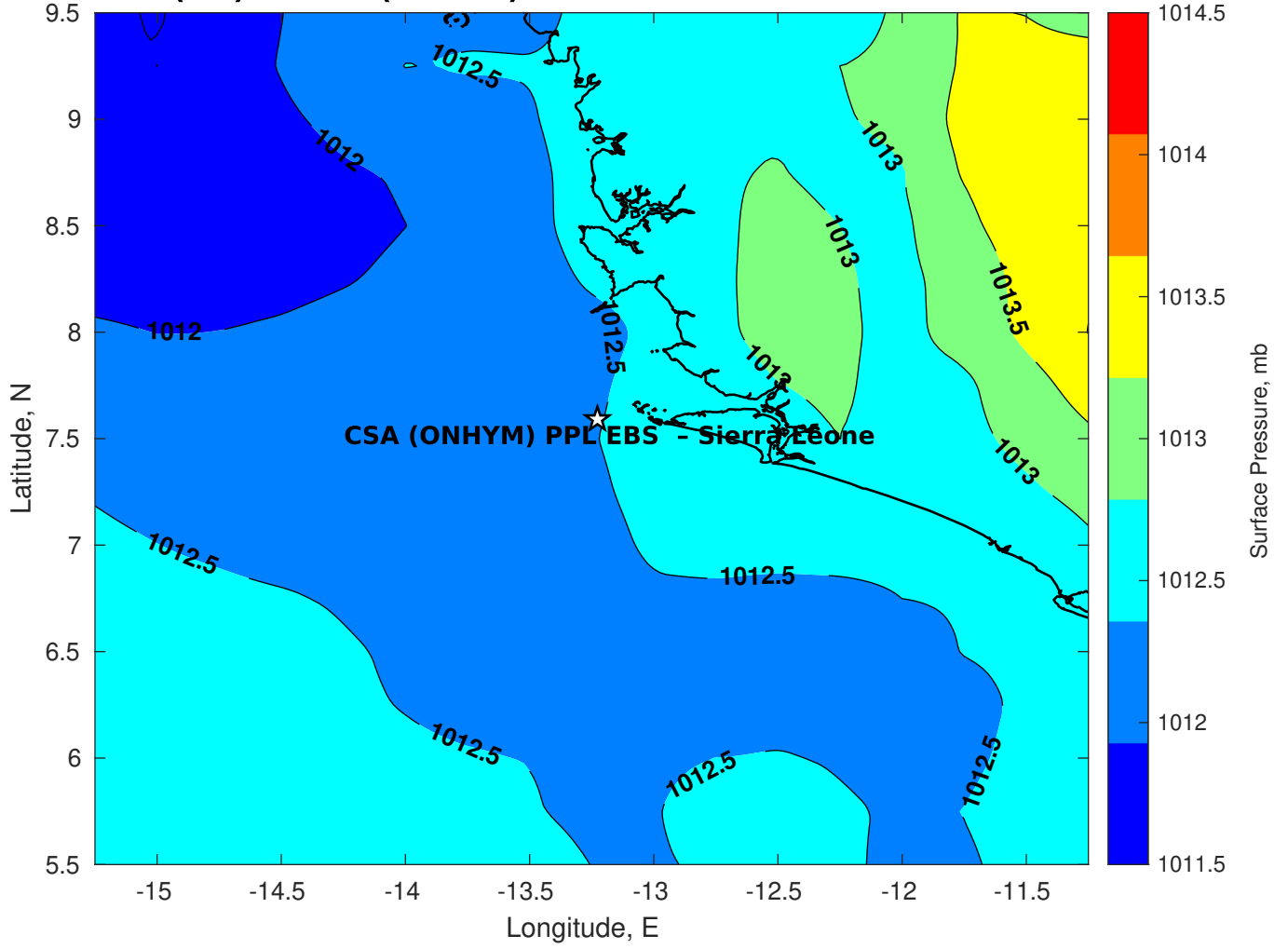
Surface Pressure (mb) for CSA (ONHYM) PPL EBS - Sierra Leone at 24-Feb-2025 00:00:00
