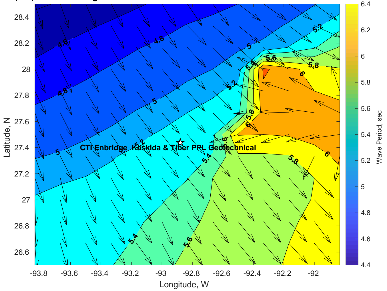
Wave Period (sec) for CTI Enbridge Kaskida & Tiber PPL Geotechnical at 24-Feb-2025 09:00:00
