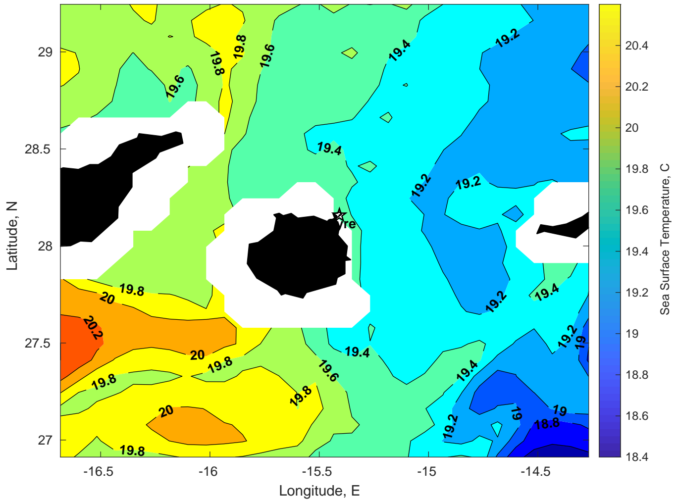
SST for Gyre at 23-Feb-2025 00:00:00
