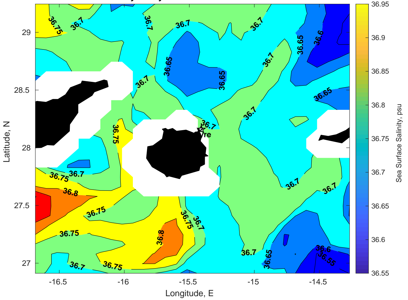
Surface Salinity for Gyre at 23-Feb-2025 00:00:00
