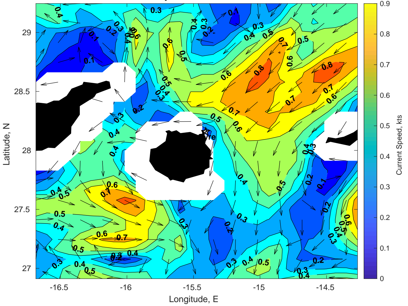
Surface Currents for Gyre at 23-Feb-2025 00:00:00
