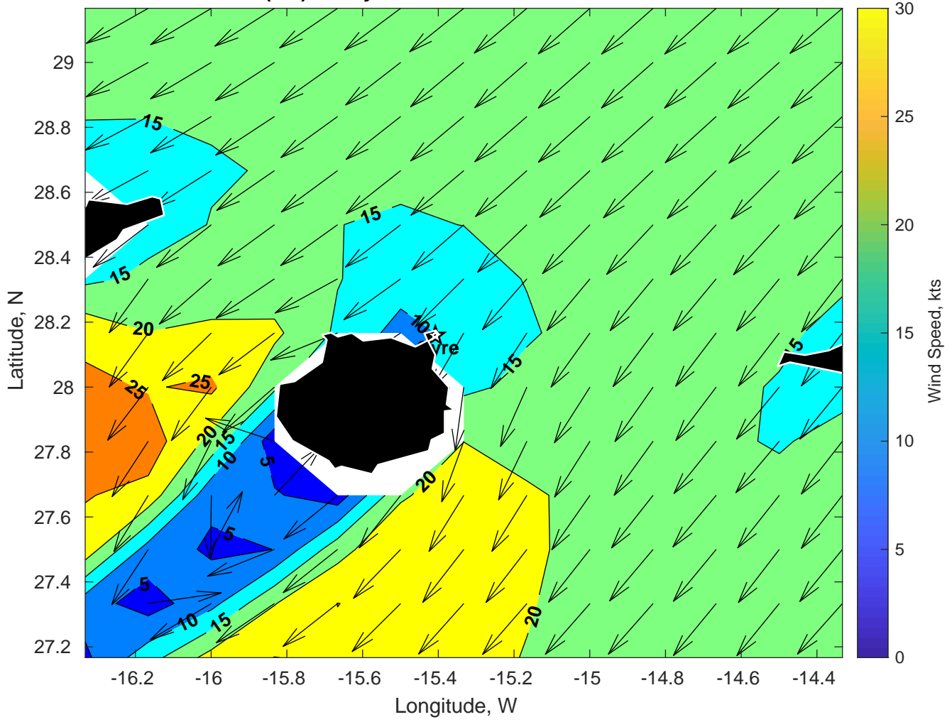
Winds (kts) for Gyre at 24-Feb-2025 09:00:00
