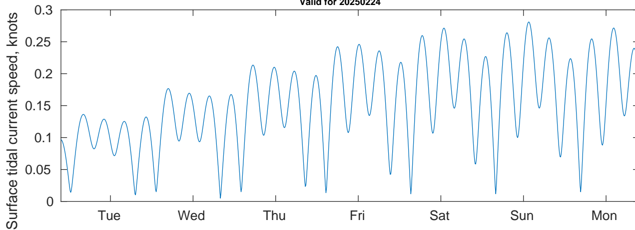
Tidal Currents and Heights for Gyre at 20250224
