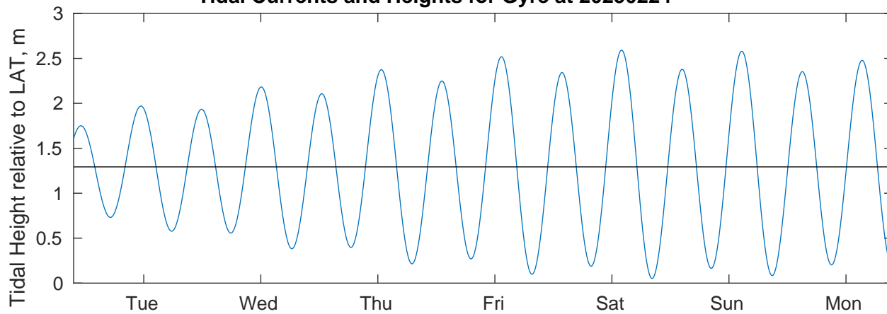
Tidal Currents and Heights for Gyre at 20250224
