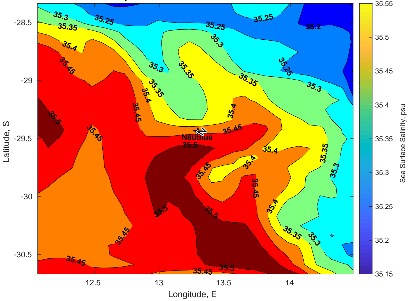
Surface Salinity for Nautilus at 23-Feb-2025 00:00:00
