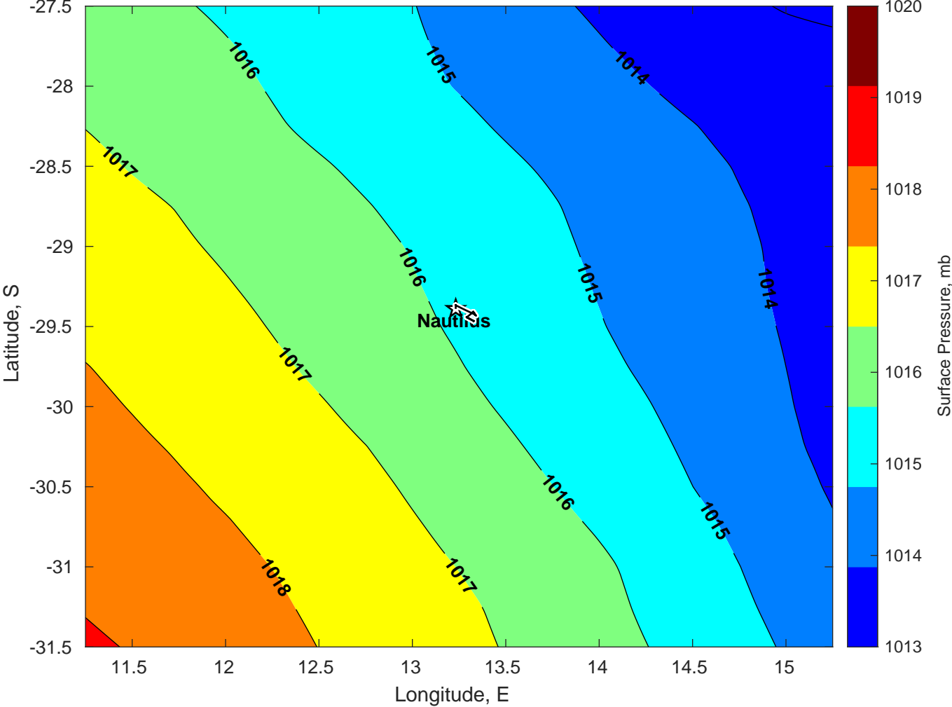
Surface Pressure (mb) for Nautilus at 26-Feb-2025 00:00:00
