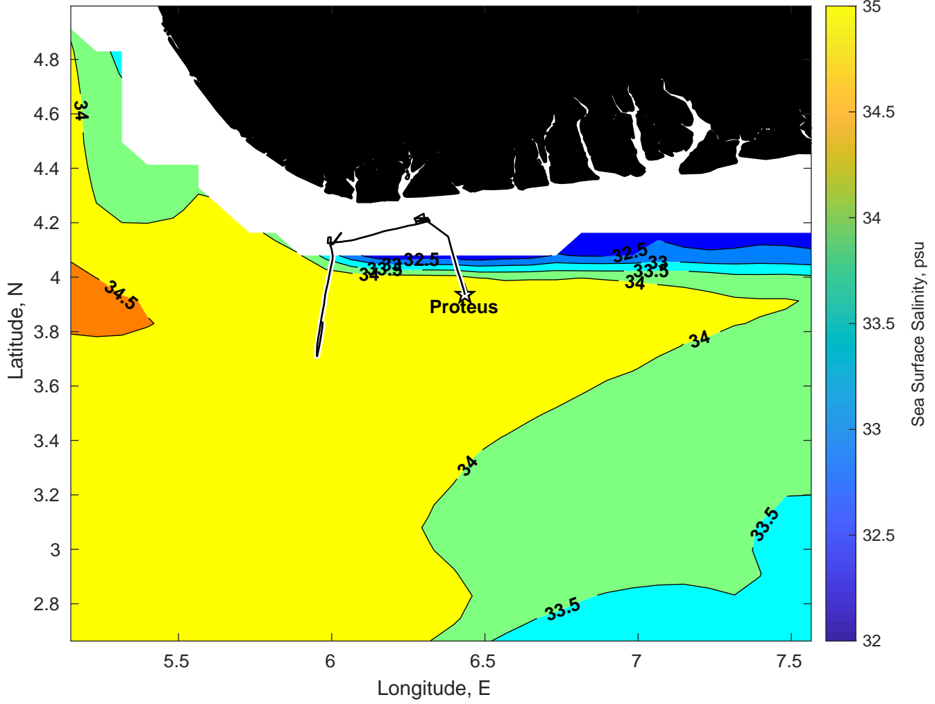
Surface Salinity for Proteus at 23-Feb-2025 00:00:00
