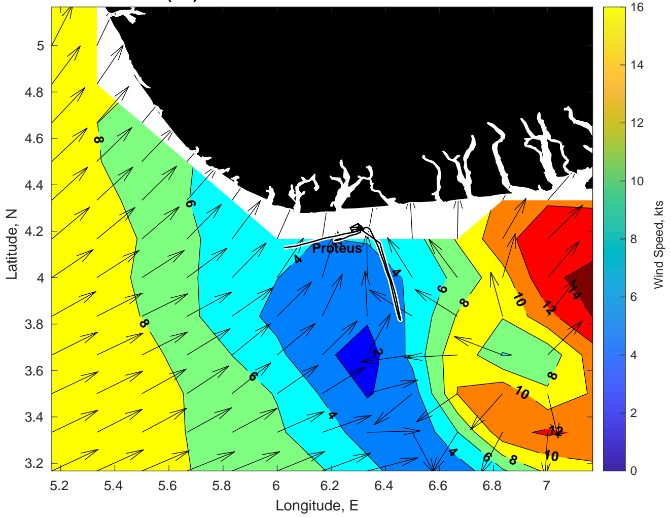
Winds (kts) for Proteus at 24-Feb-2025 09:00:00
