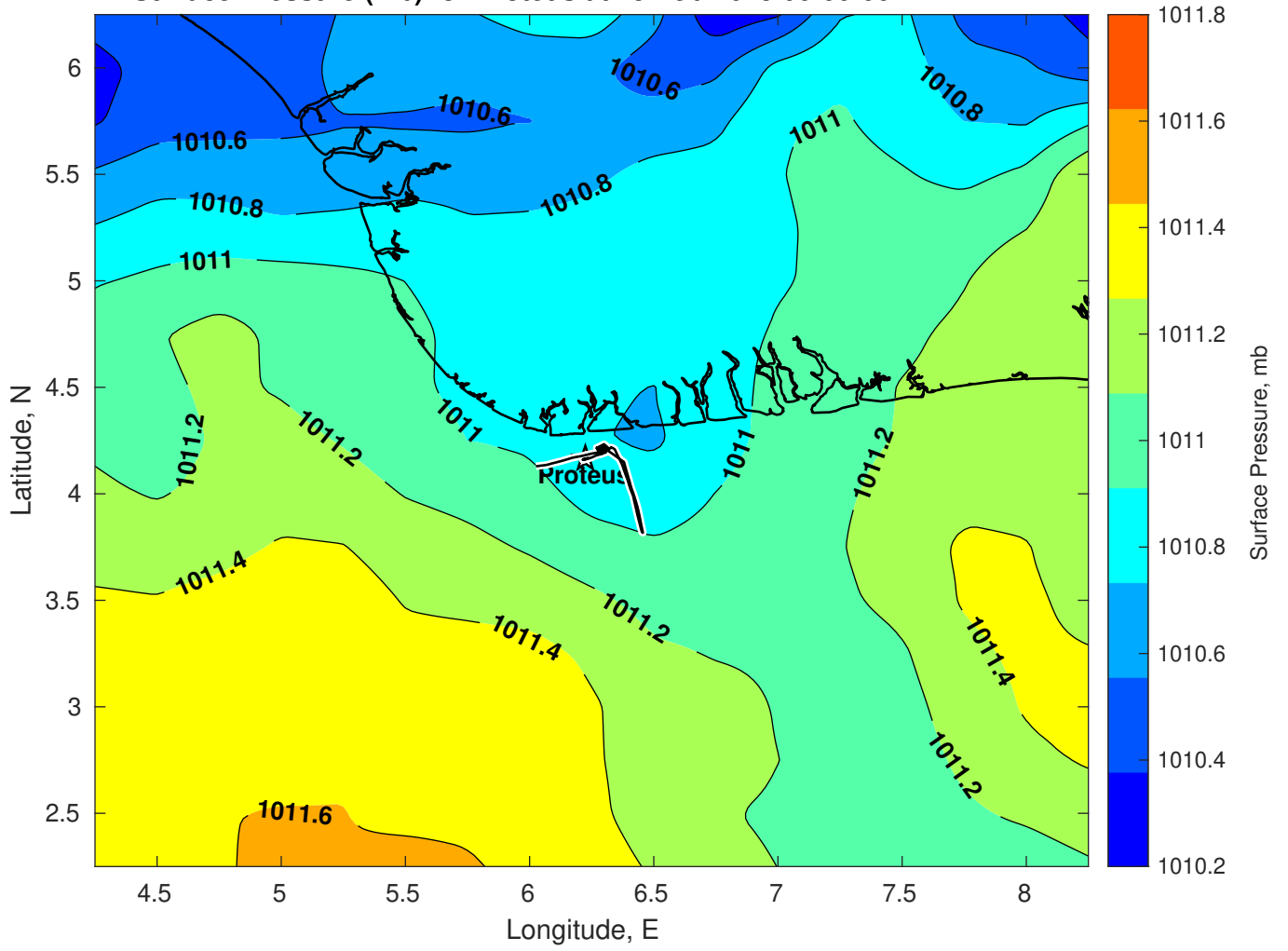
Surface Pressure (mb) for Proteus at 25-Feb-2025 00:00:00
