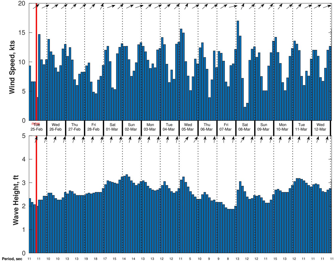
Wind & Wave Forecast for Proteus from 24-Feb-2025 01:00:00 to 12-Mar-2025 01:00:00
