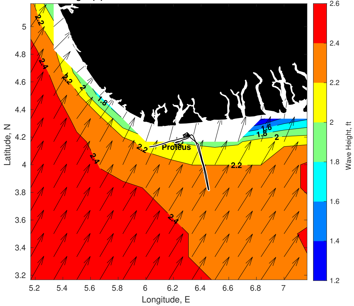
Wave Height (ft) for Proteus at 24-Feb-2025 09:00:00
