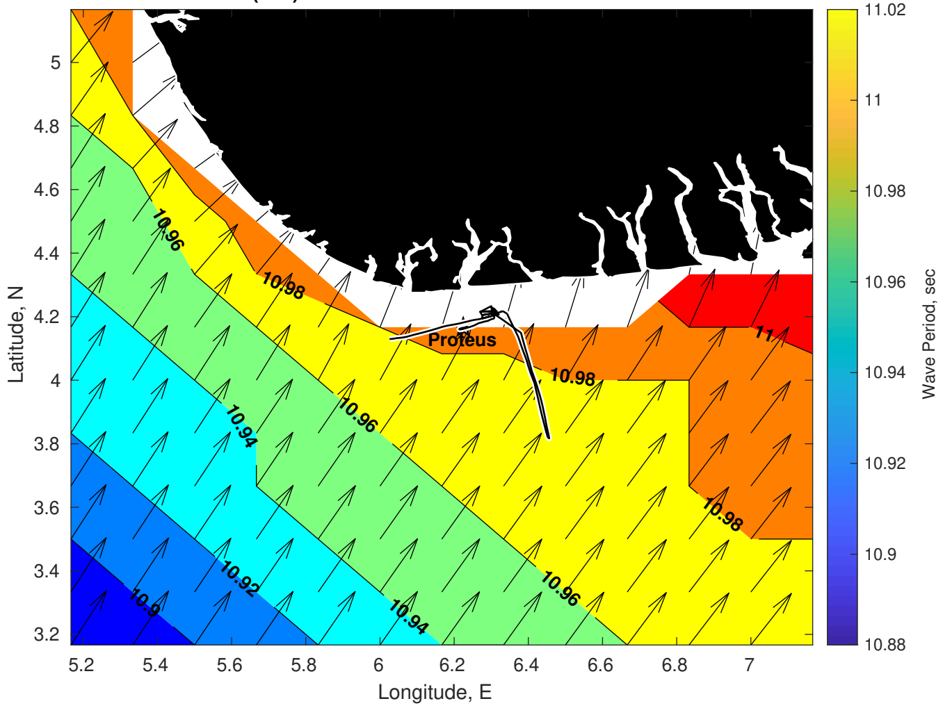
Wave Period (sec) for Proteus at 24-Feb-2025 09:00:00
