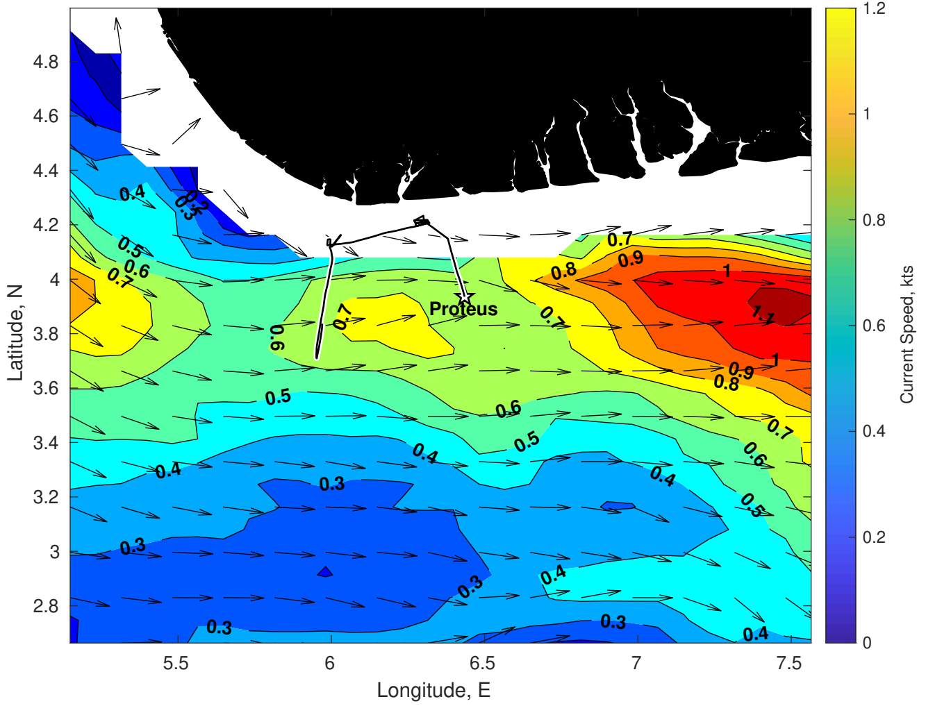
Surface Currents for Proteus at 23-Feb-2025 00:00:00
