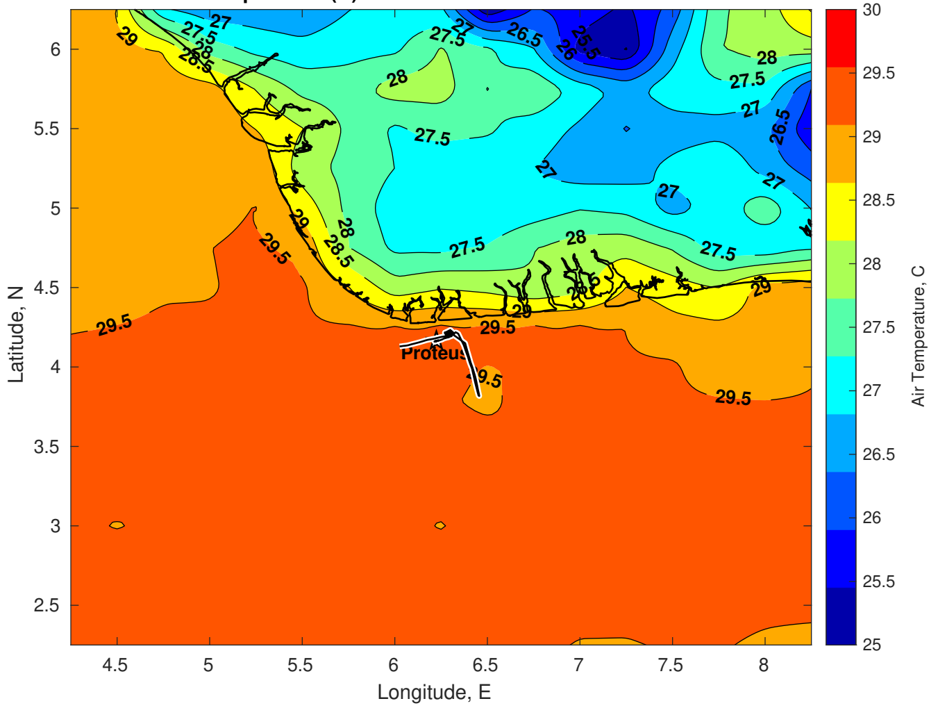
Air Temperature (C) for Proteus at 24-Feb-2025
