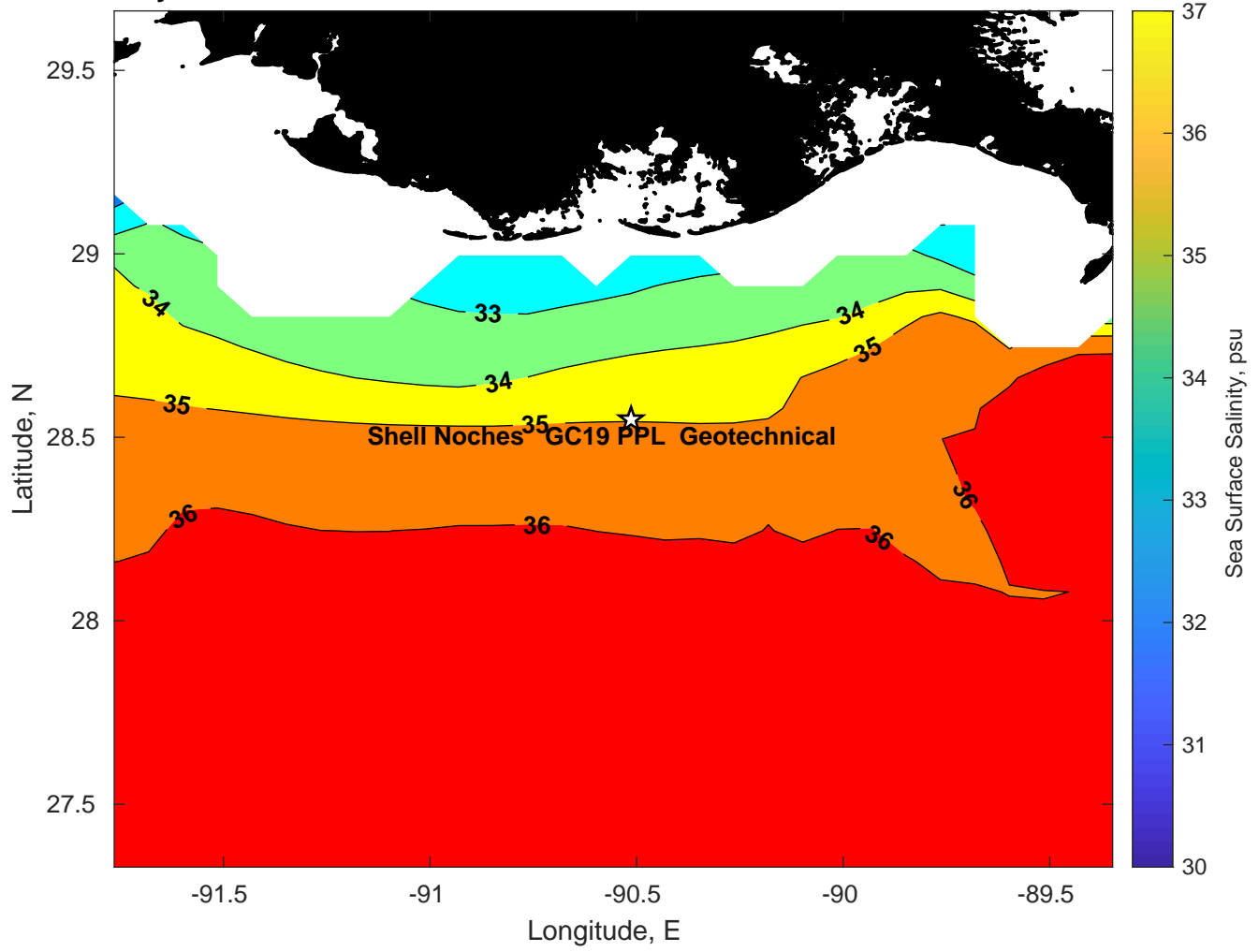
Surface Salinity for Shell Noches GC19 PPL Geotechnical at 23-Feb-2025 00:00:00
