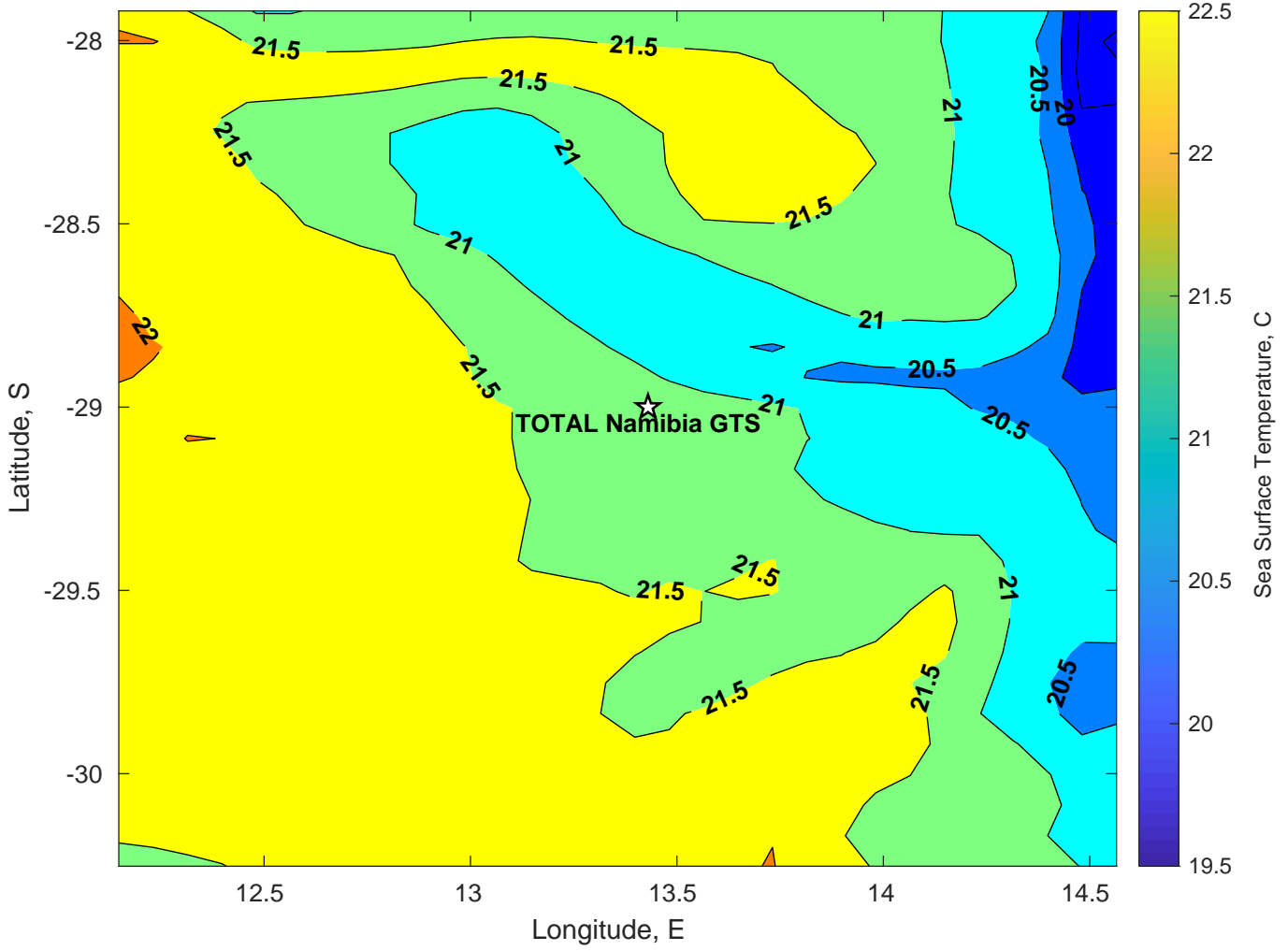
SST for TOTAL Namibia GTS at 23-Feb-2025 00:00:00
