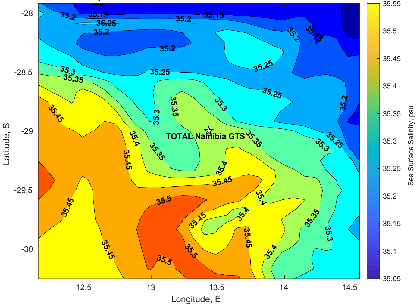
Surface Salinity for TOTAL Namibia GTS at 23-Feb-2025 00:00:00
