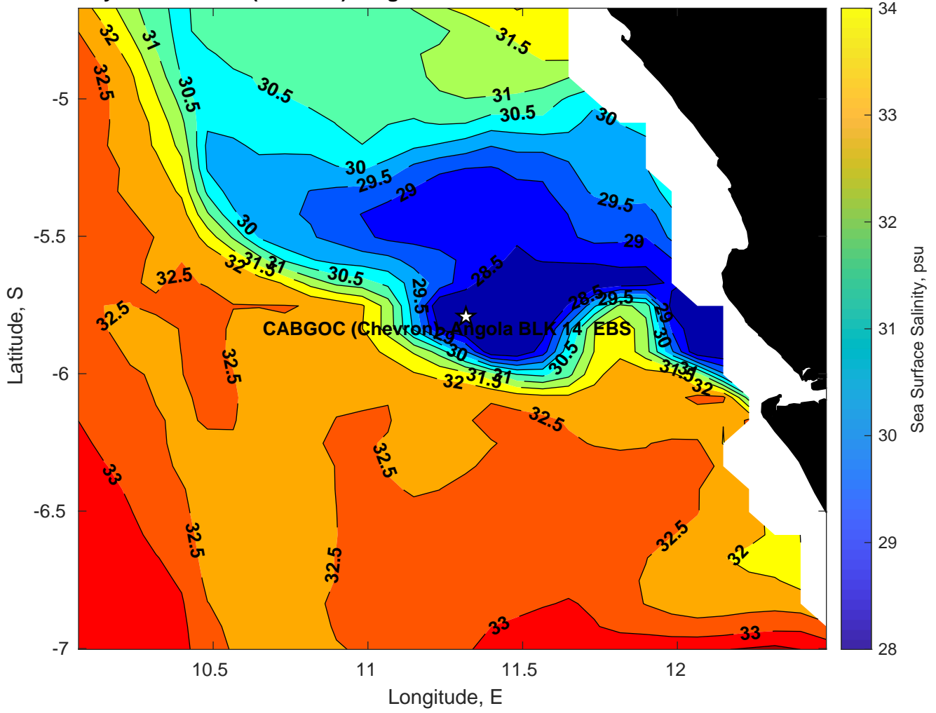
Surface Salinity for CABGOC (Chevron) Angola BLK 14 EBS at 24-Feb-2025 00:00:00
