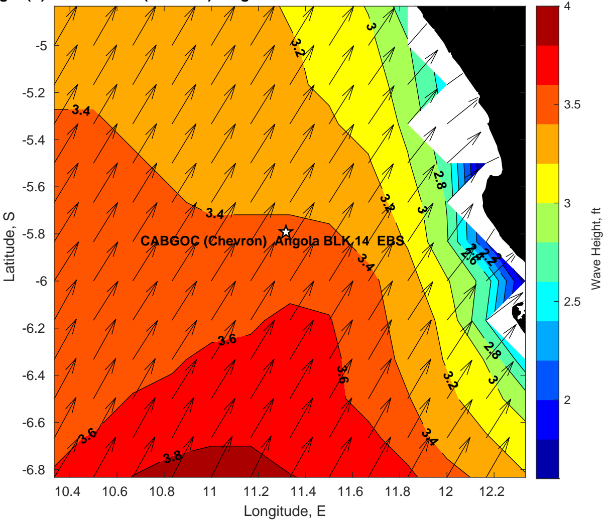
Wave Height (ft) for CABGOC (Chevron) Angola BLK 14 EBS at 25-Feb-2025 09:00:00
