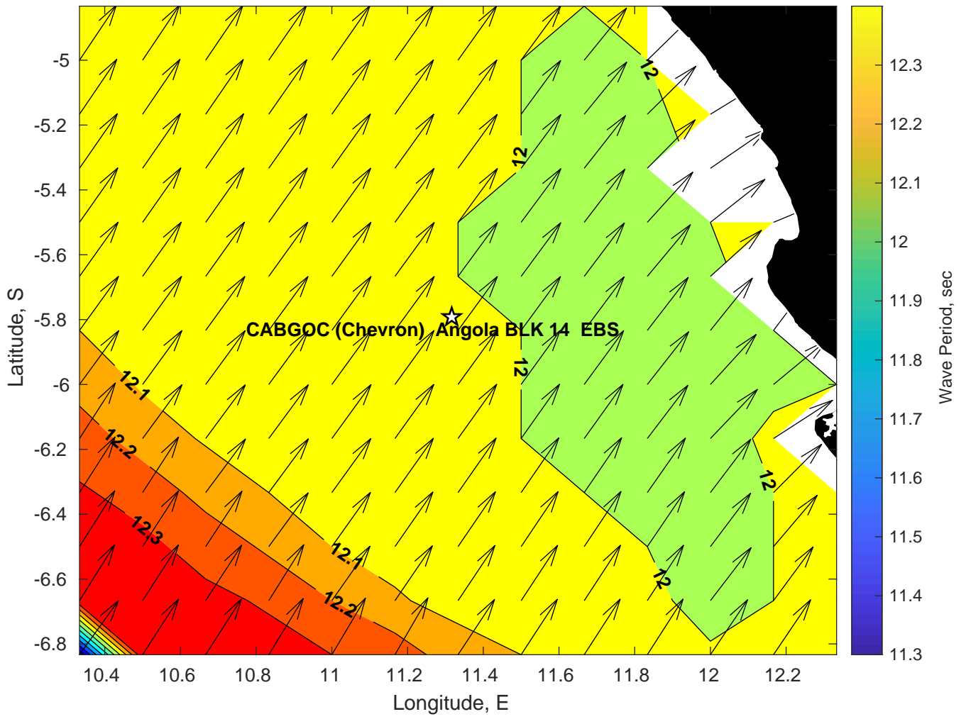
Wave Period (sec) for CABGOC (Chevron) Angola BLK 14 EBS at 25-Feb-2025 09:00:00
