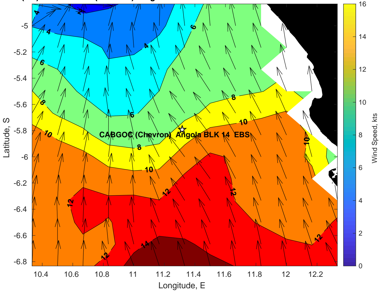
Winds (kts) for CABGOC (Chevron) Angola BLK 14 EBS at 25-Feb-2025 09:00:00
