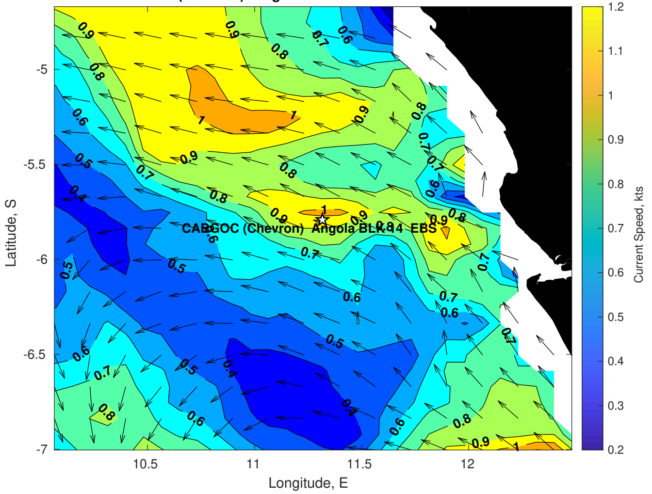
Surface Currents for CABGOC (Chevron) Angola BLK 14 EBS at 24-Feb-2025 00:00:00
