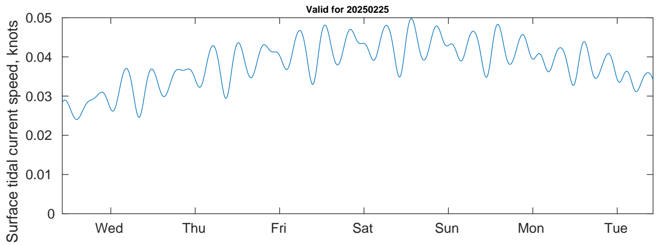
Tidal Currents and Heights for CABGOC (Chevron) Angola BLK 14 EBS at 20250225
