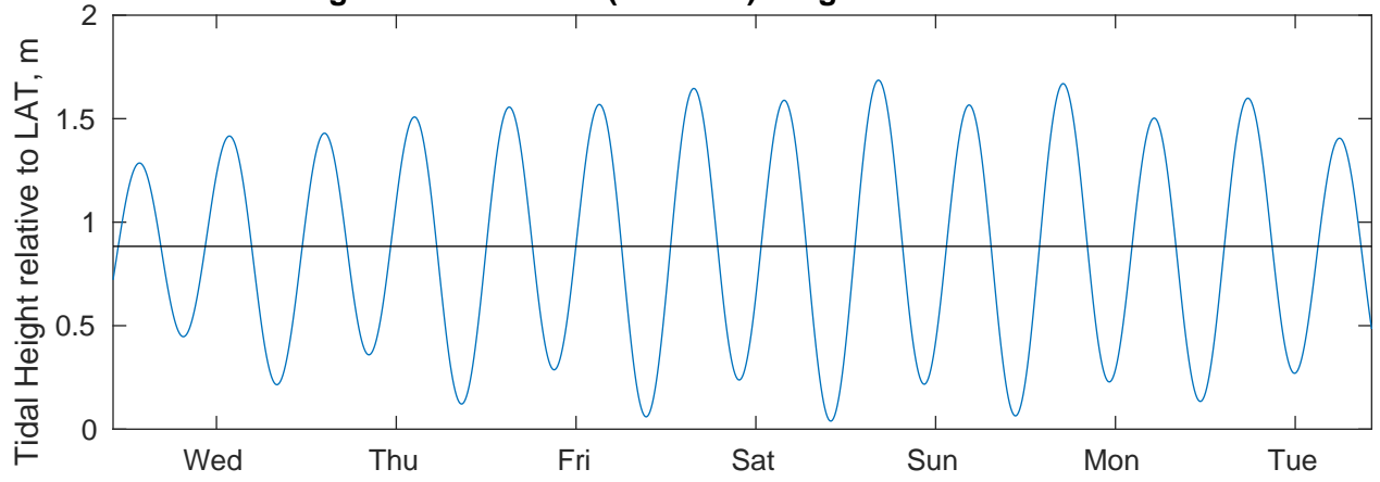
Tidal Currents and Heights for CABGOC (Chevron) Angola BLK 14 EBS at 20250225
