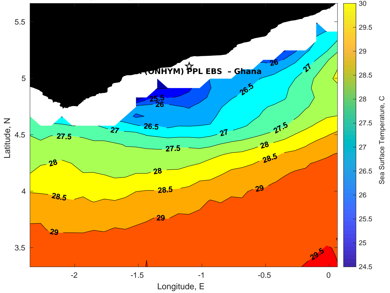
SST for CSA (ONHYM) PPL EBS - Ghana at 24-Feb-2025 00:00:00
