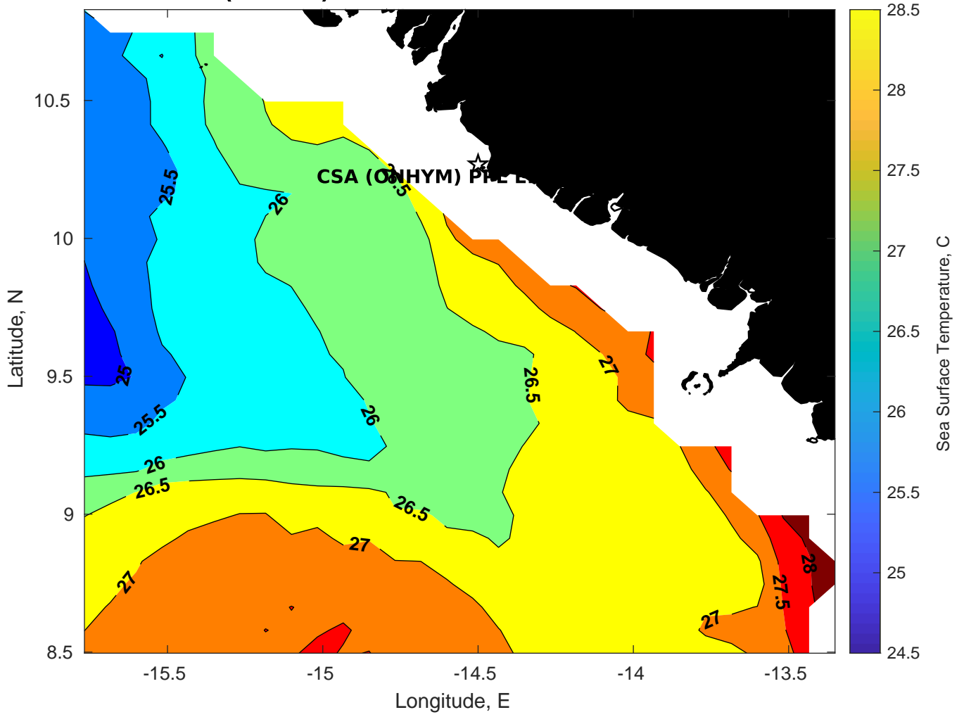
SST for CSA (ONHYM) PPL EBS - Guinea at 24-Feb-2025 00:00:00
