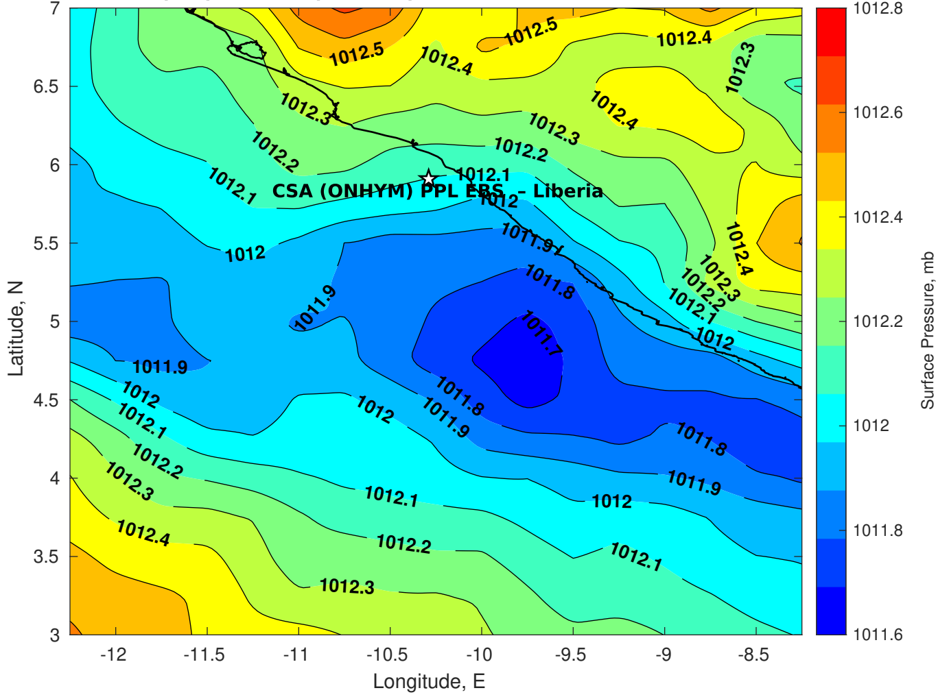
Surface Pressure (mb) for CSA (ONHYM) PPL EBS - Liberia at 27-Feb-2025 00:00:00
