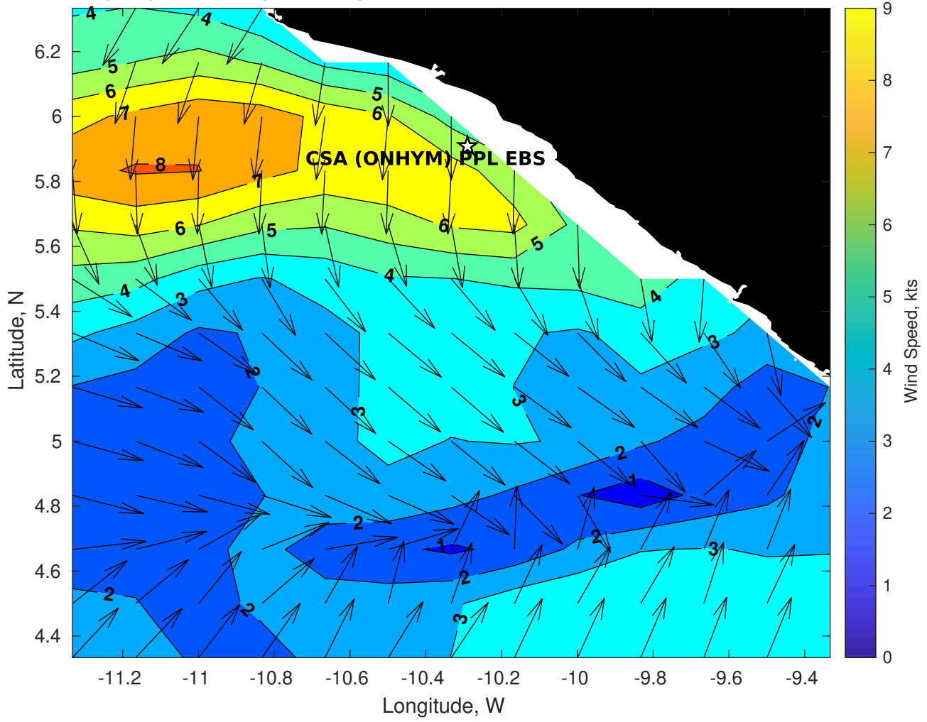
Winds (kts) for CSA (ONHYM) PPL EBS - Liberia at 25-Feb-2025 09:00:00
