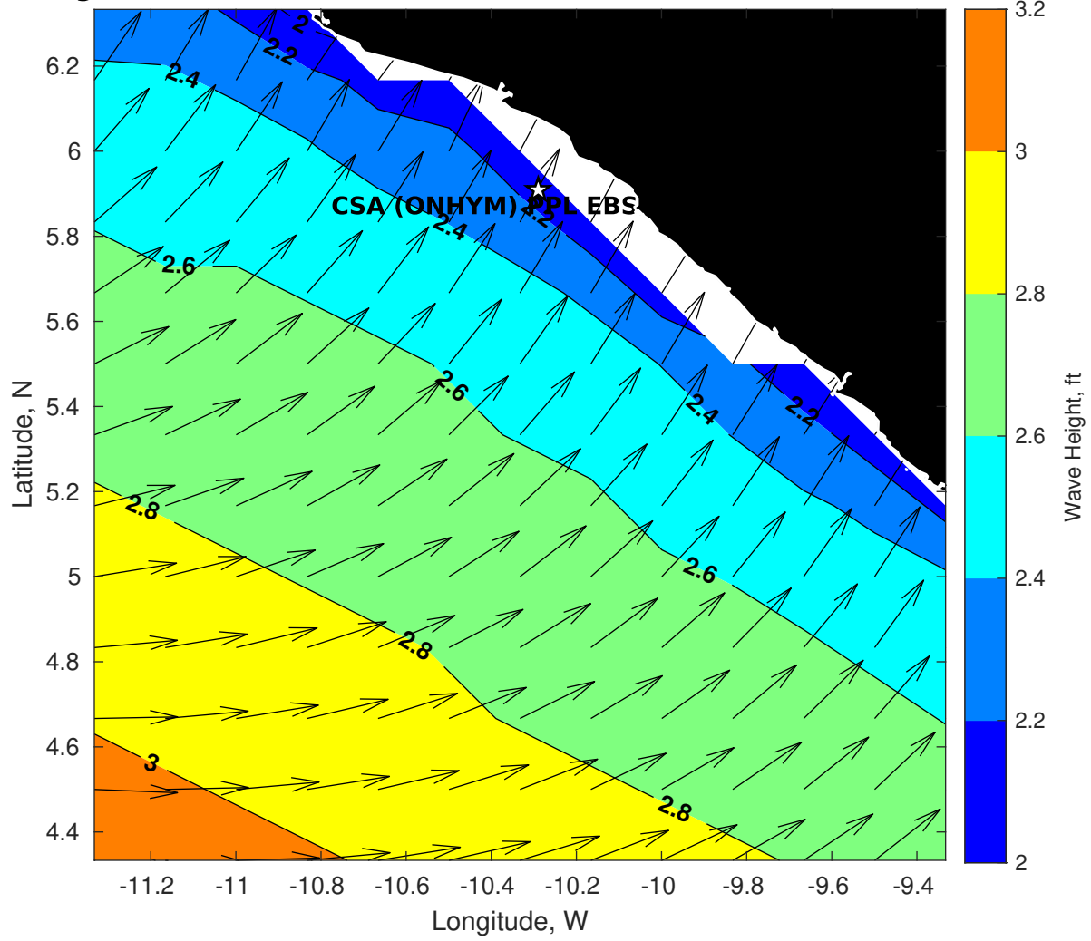
Wave Height (ft) for CSA (ONHYM) PPL EBS - Liberia at 25-Feb-2025 09:00:00
