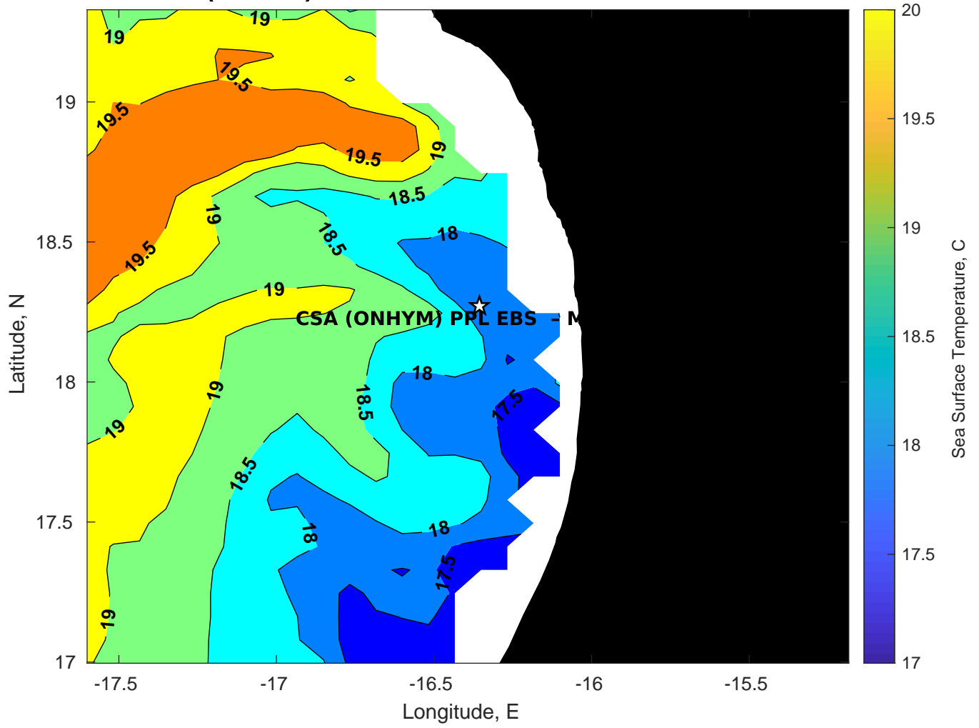
SST for CSA (ONHYM) PPL EBS - Mauritania at 24-Feb-2025 00:00:00
