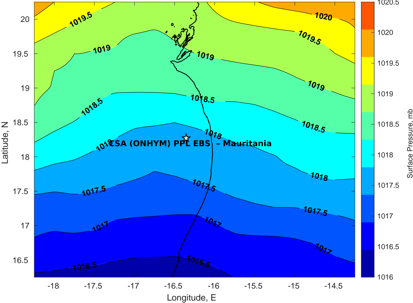
Surface Pressure (mb) for CSA (ONHYM) PPL EBS - Mauritania at 25-Feb-2025 00:00:00
