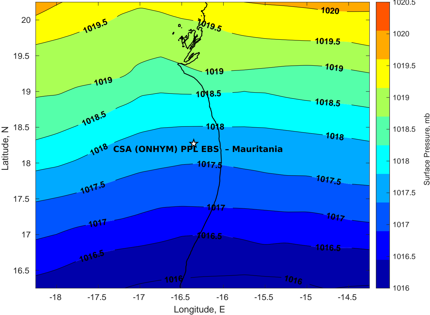
Surface Pressure (mb) for CSA (ONHYM) PPL EBS - Mauritania at 26-Feb-2025 00:00:00
