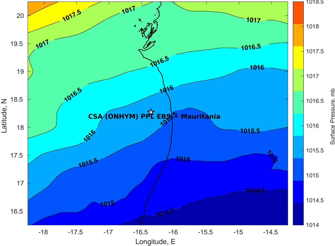
Surface Pressure (mb) for CSA (ONHYM) PPL EBS - Mauritania at 27-Feb-2025 00:00:00
