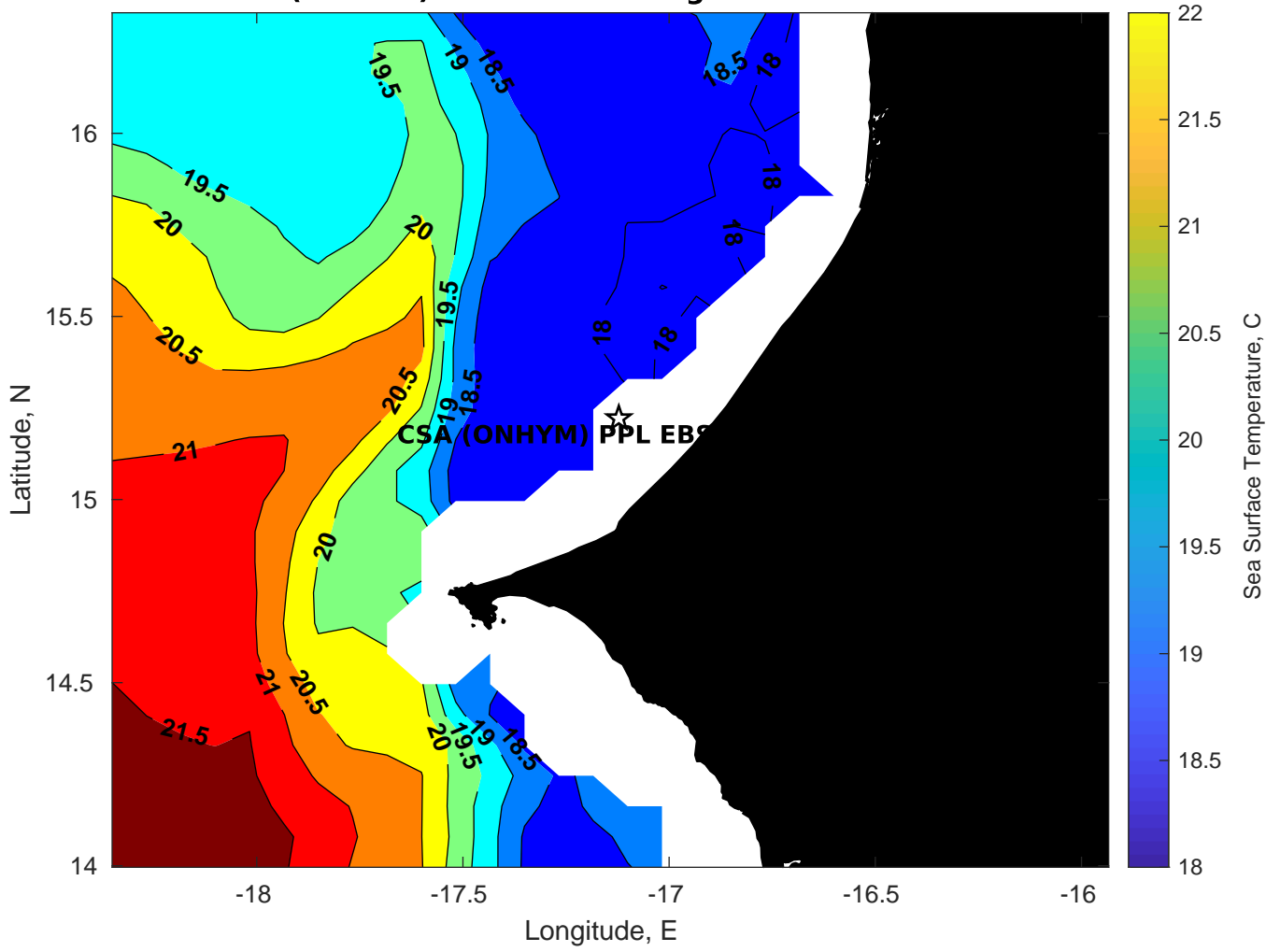
SST for CSA (ONHYM) PPL EBS - Senegal at 24-Feb-2025 00:00:00
