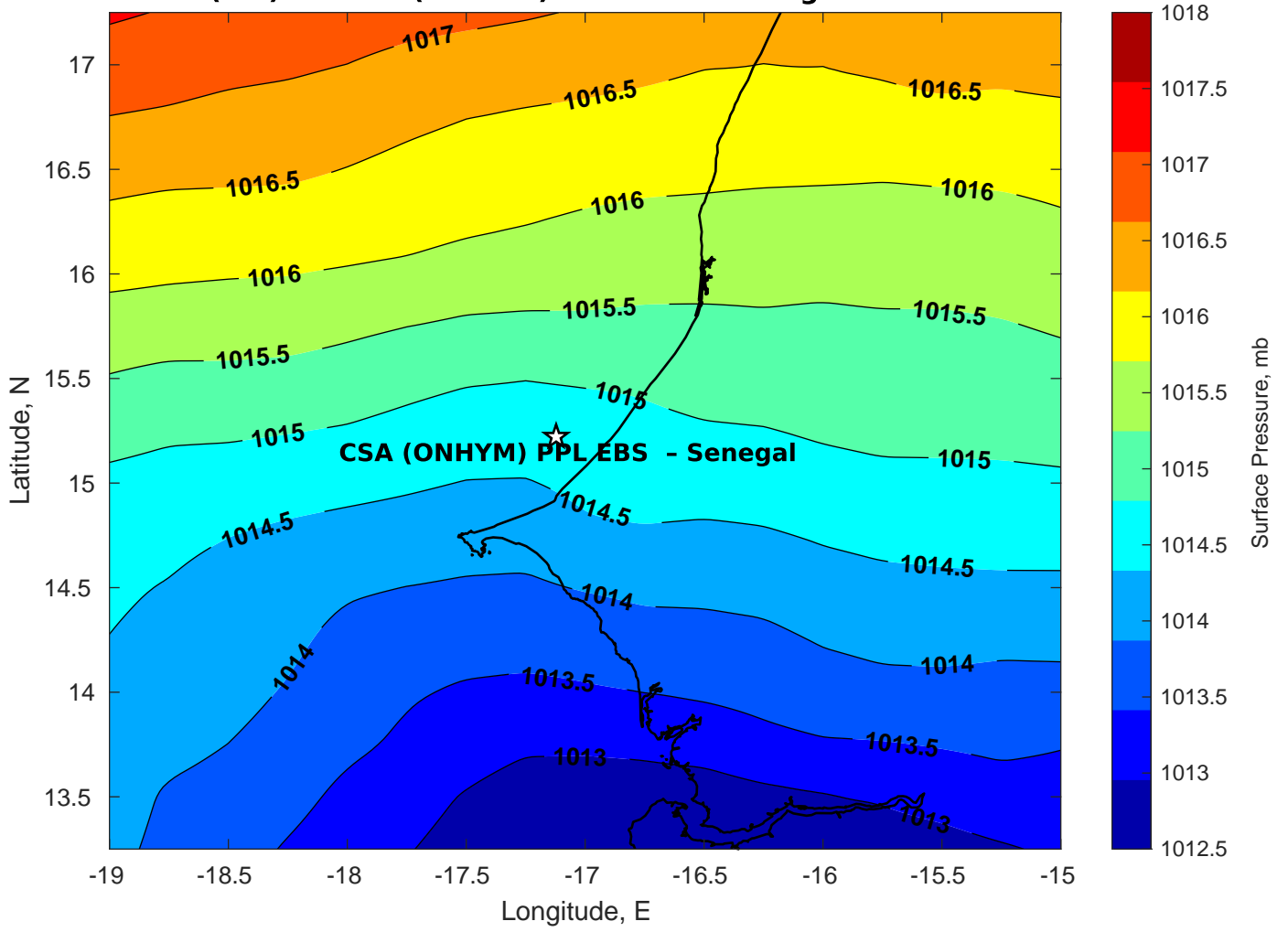
Surface Pressure (mb) for CSA (ONHYM) PPL EBS - Senegal at 26-Feb-2025 00:00:00
