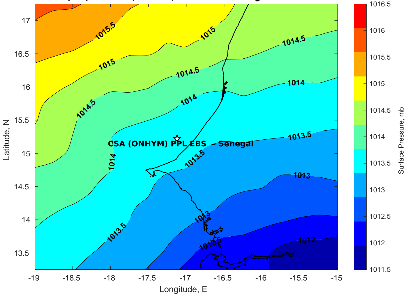
Surface Pressure (mb) for CSA (ONHYM) PPL EBS - Senegal at 27-Feb-2025 00:00:00
