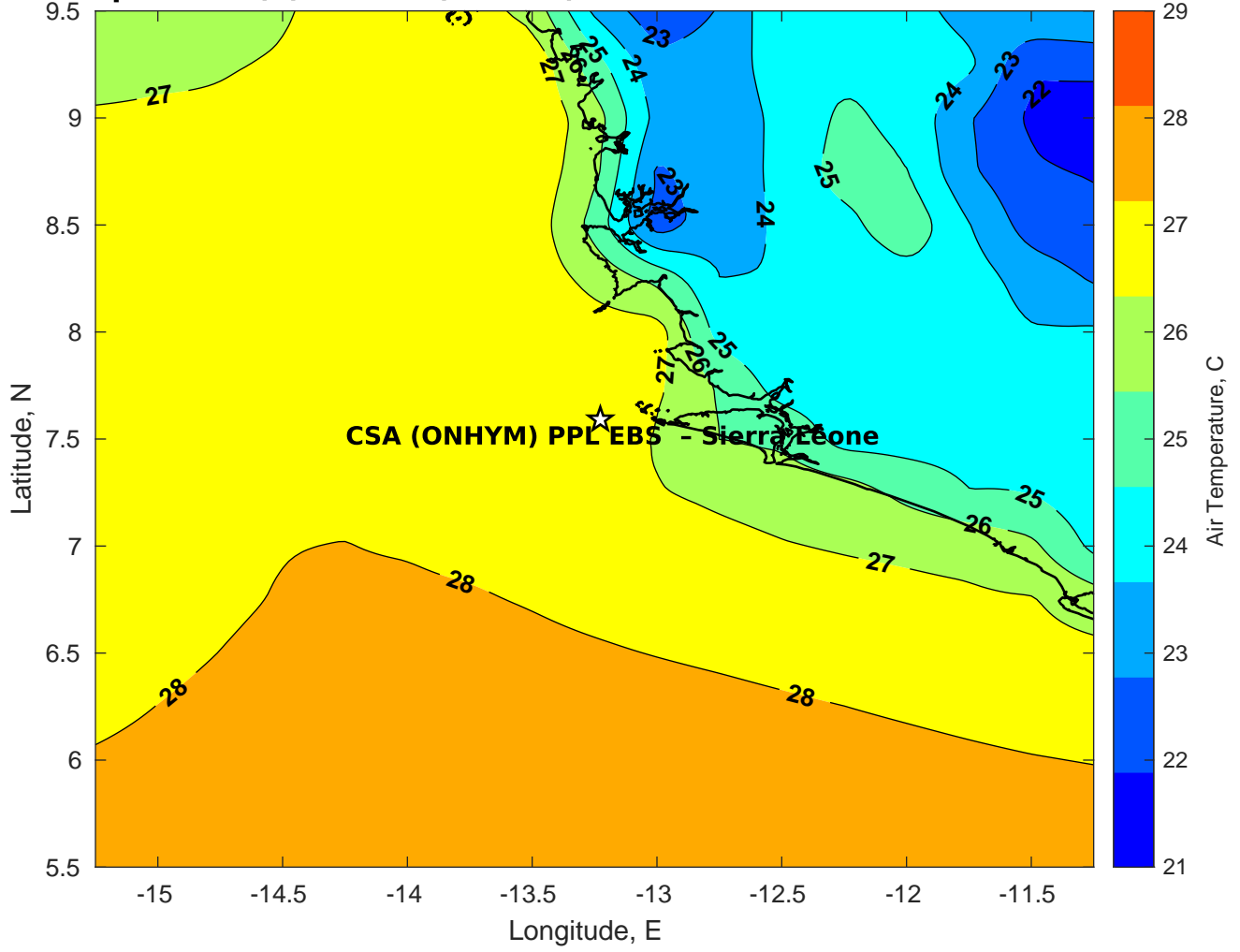
Air Temperature (C) for CSA (ONHYM) PPL EBS - Sierra Leone at 25-Feb-2025
