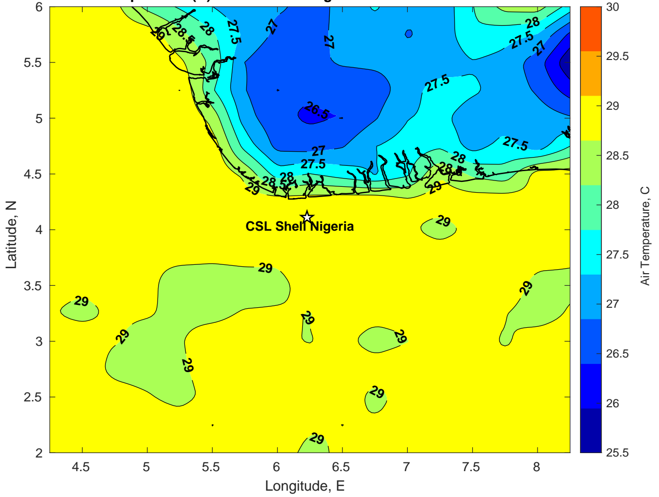
Air Temperature (C) for CSL Shell Nigeria at 25-Feb-2025
