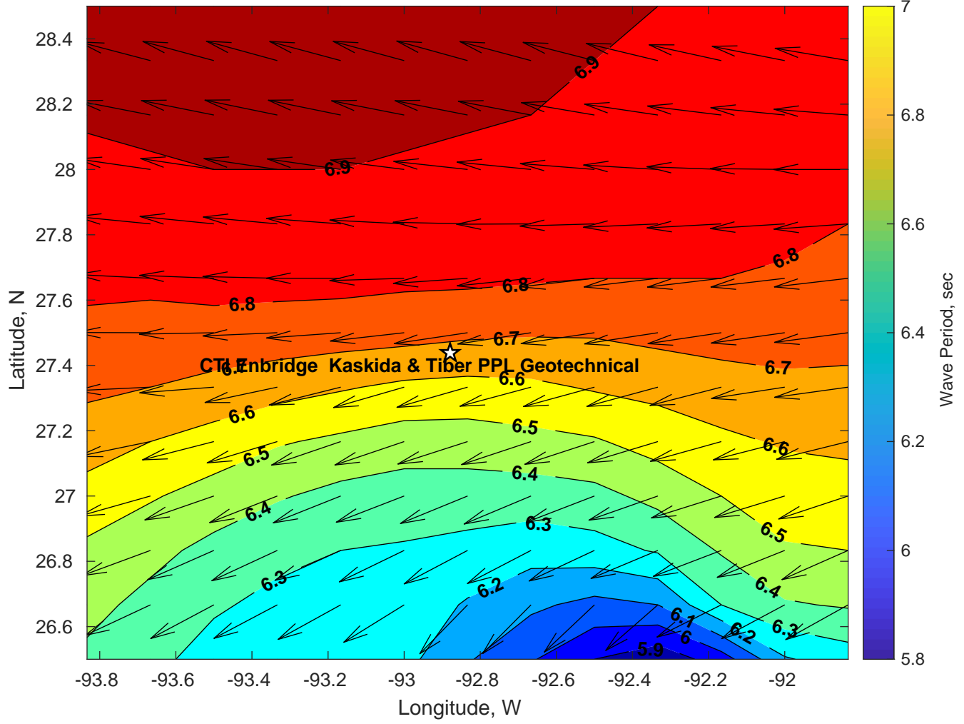
Wave Period (sec) for CTI Enbridge Kaskida & Tiber PPL Geotechnical at 25-Feb-2025 09:00:00
