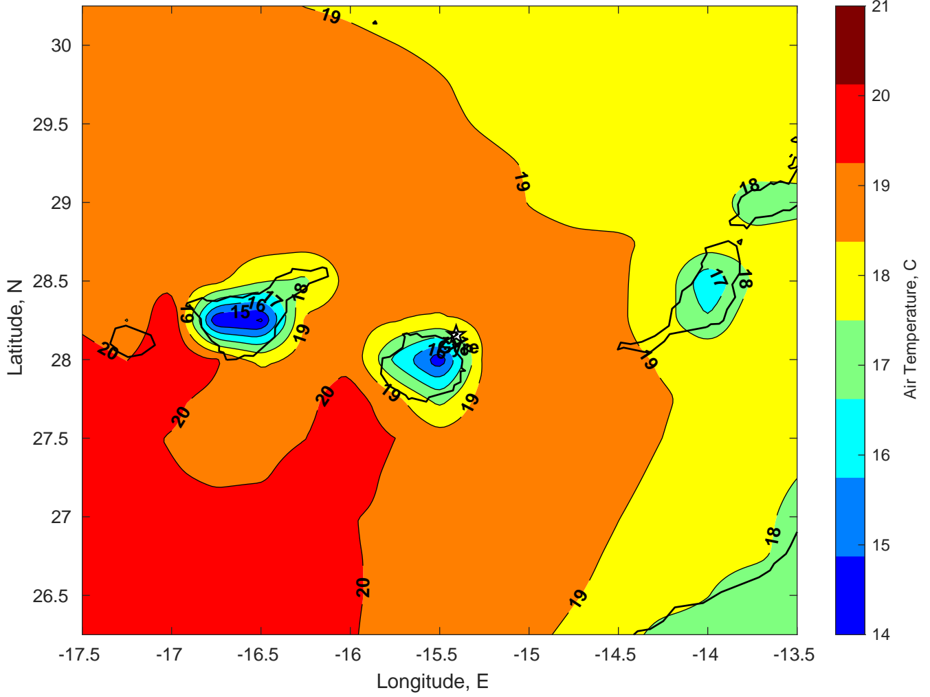
Air Temperature (C) for Gyre at 25-Feb-2025
