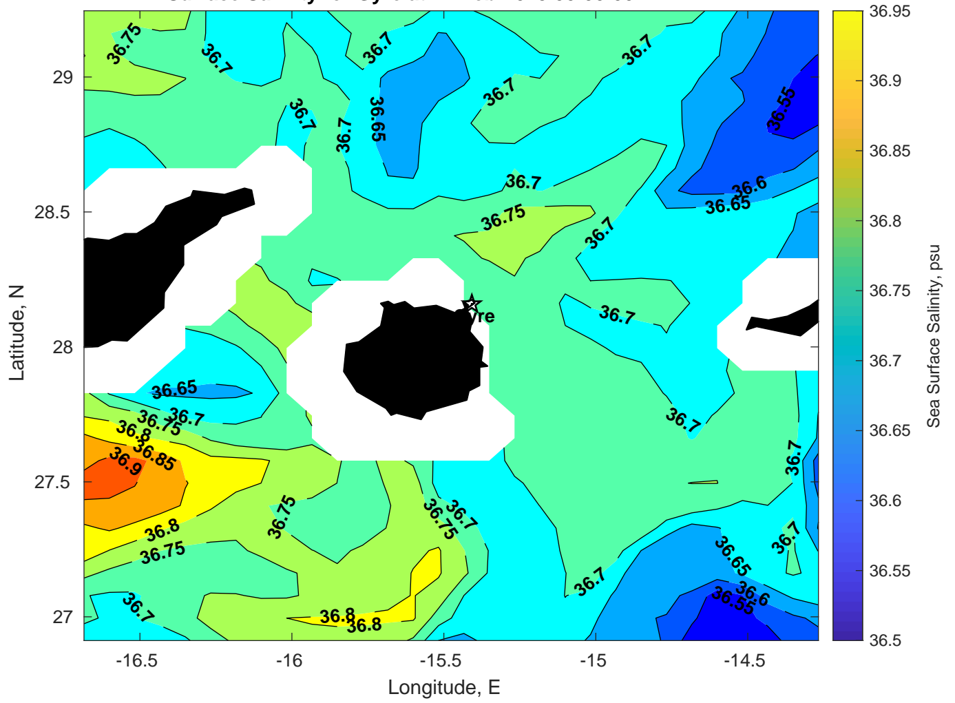
Surface Salinity for Gyre at 24-Feb-2025 00:00:00
