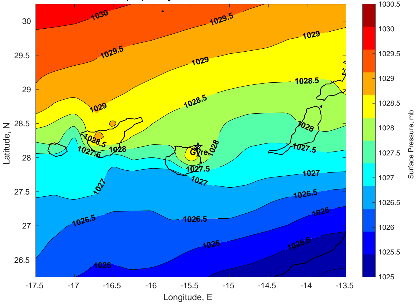
Surface Pressure (mb) for Gyre at 25-Feb-2025 00:00:00
