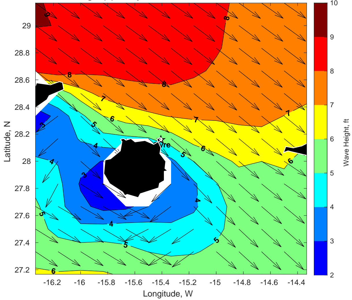
Wave Height (ft) for Gyre at 25-Feb-2025 09:00:00
