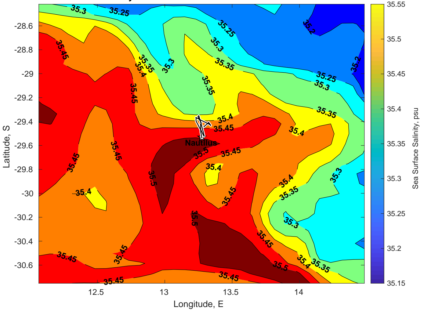
Surface Salinity for Nautilus at 24-Feb-2025 00:00:00
